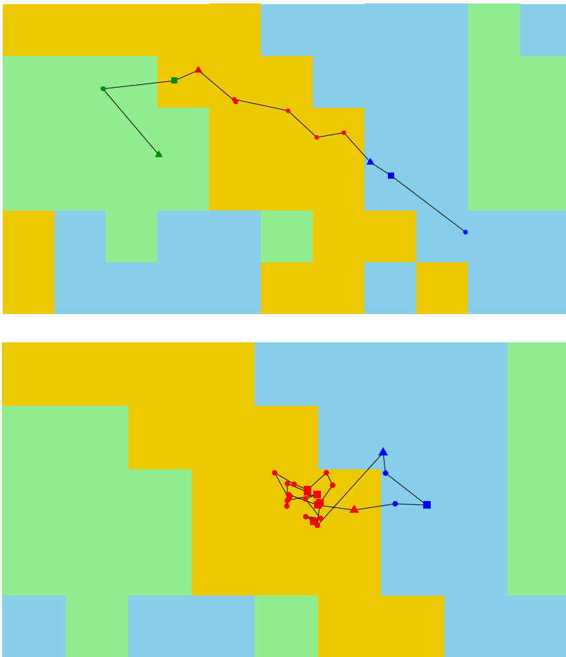
Fig. 4. Two partial reconstructed trajectories for the fisher model. Squares correspond to data points; triangles to switches in behaviour; dots to other potential switches. In part (a) (top), states 1–3 are shown in red, green, blue, respectively; in part (b) (bottom) only states 1 and 3 occur.
