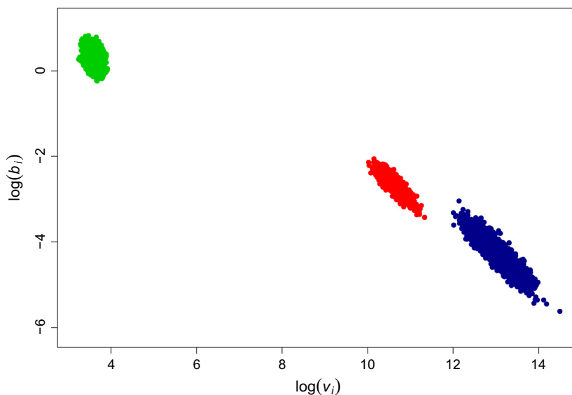
Fig. 6. State-dependent parameters for the wild boar model. The three clusters correspond to resting, returning and foraging states from left to right (green, red and blue, respectively).
