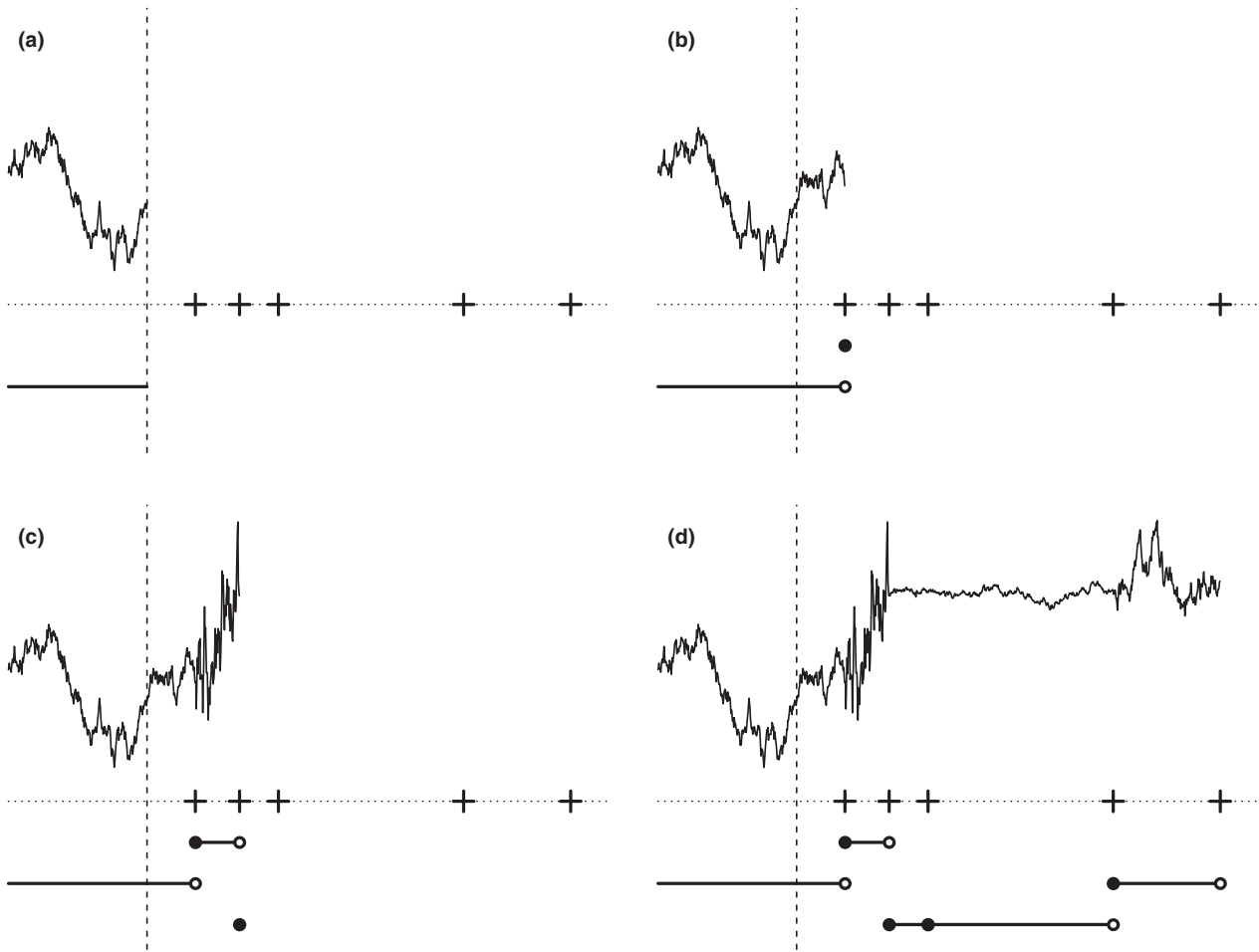
Fig. 1. Diagram of the simulation algorithm. The dotted horizontal line represents the time axis; movement is indicated in 1 dimension by the ‘noisy’ line above the time axis; behavioural state is indicated by the solid lines below. (a) The process has been simulated up to some initial time indicated by the vertical dashed line. Potential changes of state (+) are simulated as a Poisson process. (b) No change in state can occur until the first potential switch, so the process can be simulated forward in the initial state. The new location determines the probability of an actual switch. In this case, the behaviour changes from its current value (circle) to a new one (solid dot). (c) With the state for the next time interval known, the process can be simulated forward – using the new behaviour – and the next potential switch resolved. (d) This process is iterated to simulate as far as required. Here, the third potential switch shown happens not to be an actual switch.
