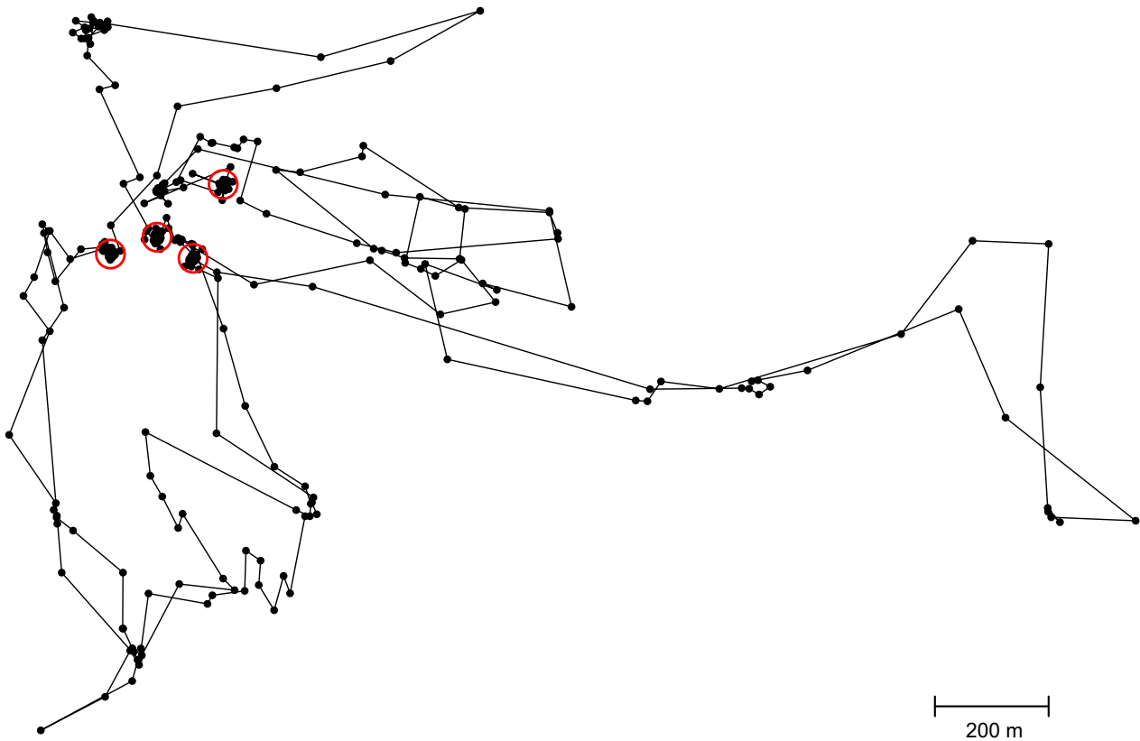
Fig. 5. Data used in wild boar example (black dots, linked in time sequence). The open red circles indicate nest locations; see text for details.
