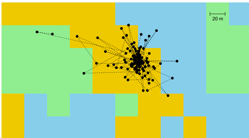
Fig. 2. Fisher locations (points, linked chronologically with dashed lines) and habitat data (coloured 30 m by 30 m grid cells). The habitats are (1) ‘developed open space’ (central band, orange); (2) ‘deciduous forest’ (mostly to the left, green) and (3) ‘woody wetlands’ (mostly to the right, blue).
