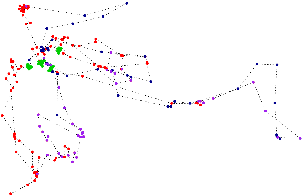
Fig. 7. Classification of observations in the wild boar model plotted in geographic space. Observations are shown here as resting (green), foraging (blue), returning (red) or uncertain (either foraging or returning – purple). See text for details.
