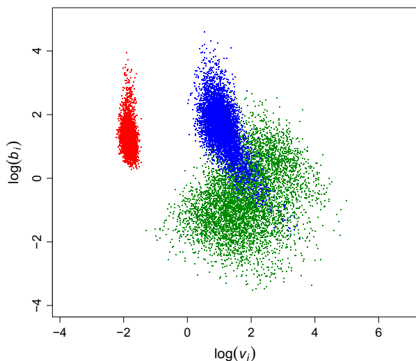
Fig. 3. State-dependent parameters for the fisher model. The three clusters correspond to states 1–3 (red, green, blue, respectively).
