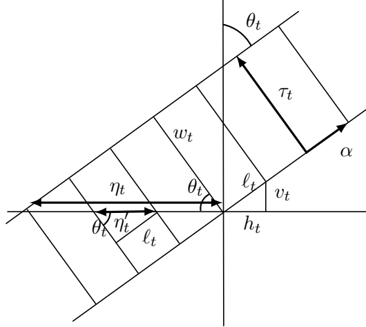
FIGURE 3. Estimating intersections in the flat annulus.
