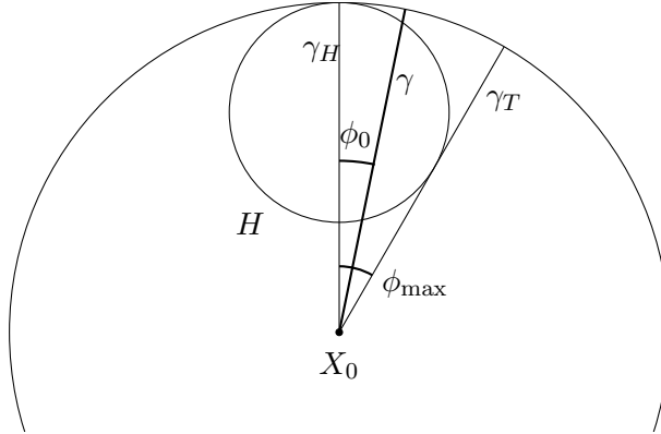
FIGURE 2. Excursion in the horoball H .
