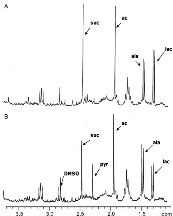
Fig. 3: 1 H nuclear magnetic resonance spectroscopy spectra of promastigote forms of Leishmania infantum . Control (A) and treated (B) with compound 5 at the concentration of IC 25 (8 \mu M). ac: acetate [singlet, 1.94 parts per million (ppm)]; ala: L-alanine (doublet, 1.5 ppm, 7.25 Hz); DMSO: dimethyl sulfoxide; lac: lactate (doublet, 1.35 ppm, 6.84 Hz); pyr: pyruvate (singlet, 2.26 ppm); suc: succinate: (singlet, 2.43 ppm).
