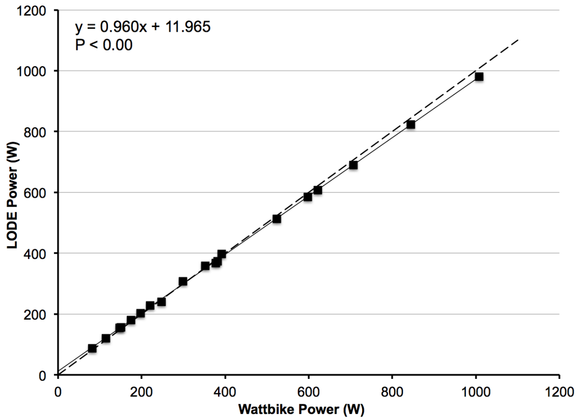
Figure 1. Scatterplot, regression model and line of identity showing the relationship between Wattbike power and LODE power for Bike 5.
