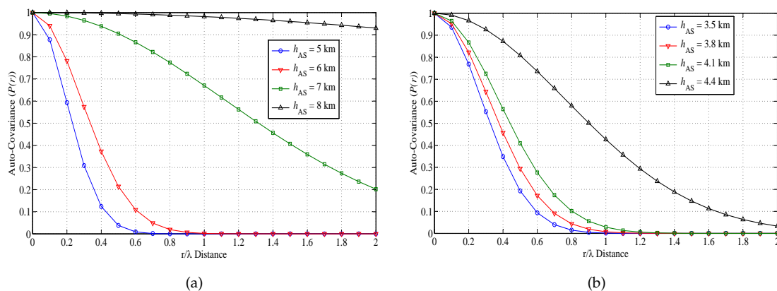
Figure 15. Auto-covariance: (a) observed from AS ( \tau_{\max} = 32 \mu\text{s} , h_{\text{CS}} = 30 \text{ m} , d = 3 \text{ km} and \sigma_c = \sigma_t = 20 \text{ m} ); (b) observed from GS ( \tau_{\max} = 25 \mu\text{s} , h_{\text{CS}} = 120 \text{ m} , d = 5 \text{ km} and \sigma_c = \sigma_t = 35 \text{ m} ).
