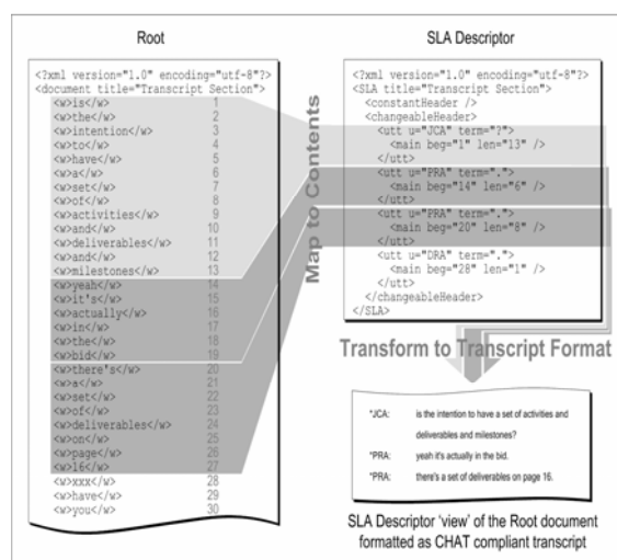
Figure 3: Reconstructing CHAT transcript from XML
