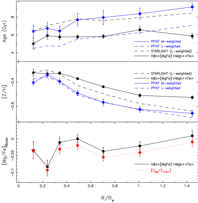
Figure 8. Age, Z , and [Mg/Fe] profiles as a function of galacto-centric radius obtained from different methods by using STARLIGHT, pPXF and index fitting. Results from STARLIGHT and pPXF are presented as black and blue lines respectively, index fitting is indicated by filled black circles, and the [Z_{Mg}/Z_{Fe}]_{Base} values are shown by the red line. The filled star in each panel indicates the NSC-contaminated bin.
