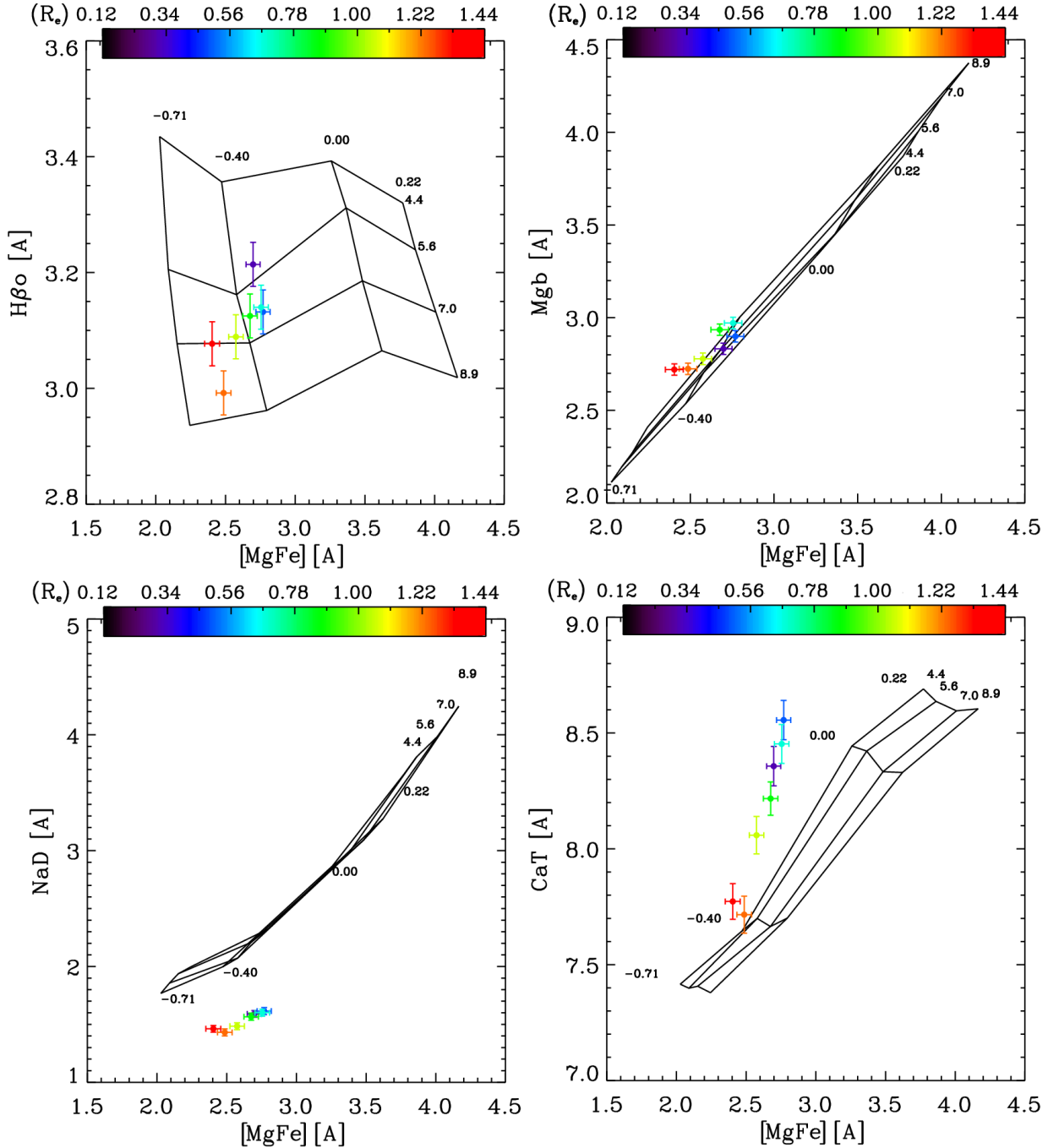
Figure 12. Index-index diagrams of H\beta_0 , Mgb , NaD , and CaT as function of total metallicity [MgFe] . MIUSCAT models grids are plotted with IMF slope of 1.3, age ranging between 4.4 Gyr to 8.9 Gyr and metallicity ranging between -0.71 to 0.22 dex. The colour coding indicates the radial distance in R/R_e where red indicates the most distant radial bin from the centre.
