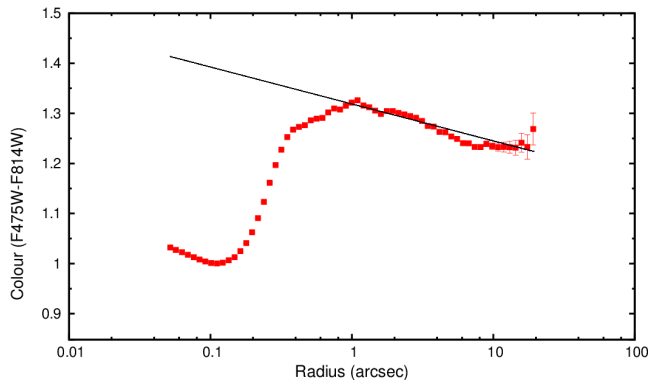
Figure 17. Colour Profile of NCG 1396 from HST archive data, with a gradient fit of -0.077 \pm 0.006 to the region outside of the central 1 arcsec. The central 0.2 arcsec is dominated by a nuclear star cluster.
