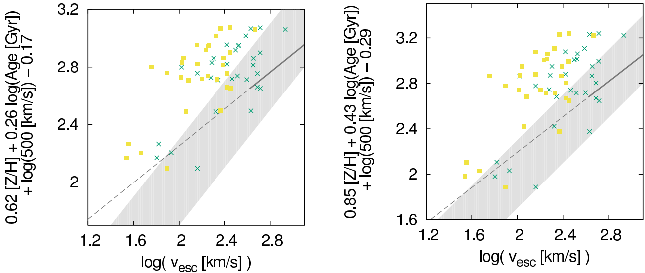
Figure 7. SSP-equivalent stellar population parameters and escape velocity. The two panels show the edge-on projections of the planes that Scott et al. (2013) , (left) and Scott et al. (2009) , (right) found to be spanned by the local stellar population parameters and escape velocities in early-type galaxies. The grey shaded regions indicate these planes \pm 0.3 dex, which is chosen by eye to generously describe regions that were populated by the profiles in these studies. For our CSSs we calculate the corresponding linear combinations of luminosity weighted age and metallicities and lower (yellow boxes) and upper (green crosses) limits for the luminosity weighted escape velocities (see text). The grey lines indicate the relations found by Scott et al. (2013) and Scott et al. (2009) for escape velocities above 400 \text{ km s}^{-1} , where the authors found the scatter to be considerably smaller. The CSSs fall on average well above the planes and relations for early-type galaxies, suggesting that their enrichments exceed what is possible for their current potential wells.
