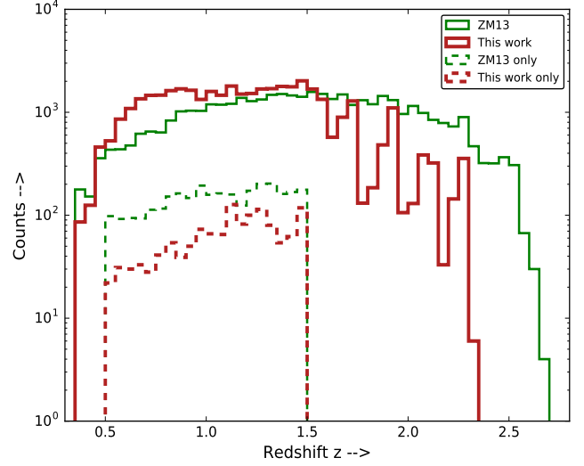
Figure 10. The redshift distributions of the absorption systems in the ZM13 (green) and the current work (red) after removing the plausible C IV systems. The dashed lines show the systems that are unique in each catalogue in the redshift range 0.5 \leq z_{2796} \leq 1.5 .
