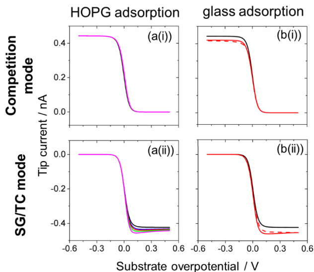
Figure 5. Simulated nanogap substrate voltammetry SECM tip current-substrate potential responses for: (a) varying values of \Gamma_{\text{HOPG,FcTMA}^+} ( 1.1 \times 10^{-10} (22 %), 1.53 \times 10^{-10} (30 %), 2.0 \times 10^{-10} (40 %) and 2.6 \times 10^{-10} (50 %) mol cm -2 ); and (b) full adsorption model (red). In both parts, the black curves represent the adsorption-free tip response. Solid and dashed lines show the forward and reverse curves, respectively. Simulation parameters: L = 0.1 , k^0 = 5 \text{ cm s}^{-1} , \nu = 50 \text{ mV s}^{-1} , a_{\text{UME}} = 0.5 \text{ }\mu\text{m} , \text{RG} = 2 , \alpha = 0.5 , D_{\text{FcTMA}^+} = 6.7 \times 10^{-6} \text{ cm s}^{-1} and D_{\text{FcTMA}^{2+}} = 6.1 \times 10^{-6} \text{ cm s}^{-1} . Glass adsorption parameters are given by \Gamma_{\text{glass}}^0 = 2.3 \times 10^{-9} \text{ mol cm}^{-2} , K_{\text{ads,glass}} = 2.56 \times 10^6 \text{ cm}^3 \text{ mol}^{-1} and K_{12} = 9 \times 10^6 \text{ M}^{-1} \text{ s}^{-1} .
