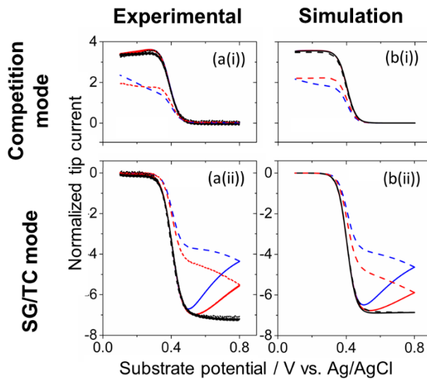
Figure 4. Experimental (a) and simulated (b) tip current-substrate potential curves for the competition and SG/TC modes for the one-electron oxidation of 0.4 mM FcTMA + in 1 M KCl supporting electrolyte in aqueous media at an HOPG surface (ZYA grade) at different scan rates (50 (blue), 100 (red), 500 (black) mV s -1 ) at L = 0.209 . Solid and dashed lines show the forward and reverse curves, respectively.
