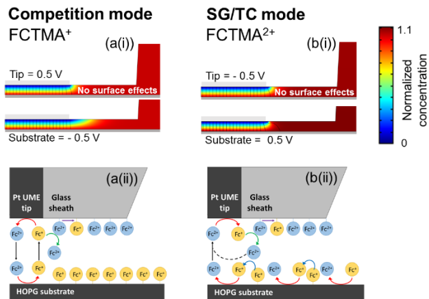
Figure 6. (i) Concentration profiles of (a) \text{FcTMA}^+ in the competition mode and (b) \text{FcTMA}^{2+} in the SG/TC mode, with the parameters defined in Figure 5 (b). (ii) Illustrations of the redox adsorption processes occurring in the (a) competition and (b) SG/TC modes.
