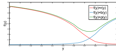
FIG. 5. Example II: Red and blue particle density as well as their sum \rho at time T = 100 in the case of nonequal initial mass.
