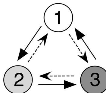
FIG. 4. Quotient network for the pattern of synchrony in Figure 3.
