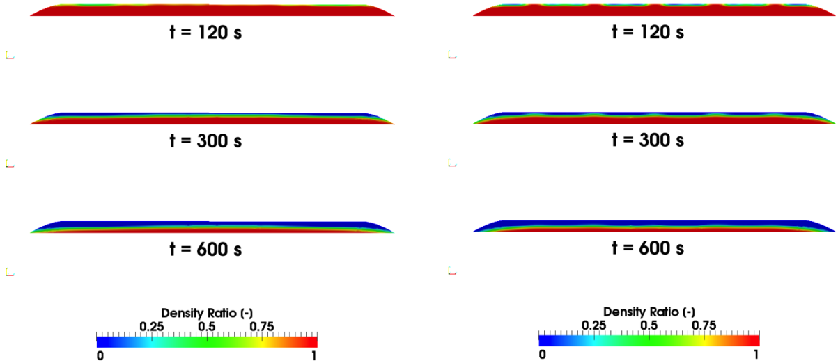
Figure 9. Density ratio fields at t = 120, 300, 600\text{ s} for \theta = 90^{\circ} (left) and 180^{\circ} (right). Note: The figure is zoomed-in to capture only the affected area in the CFRP material (the plastic liner and metallic boss are omitted).
