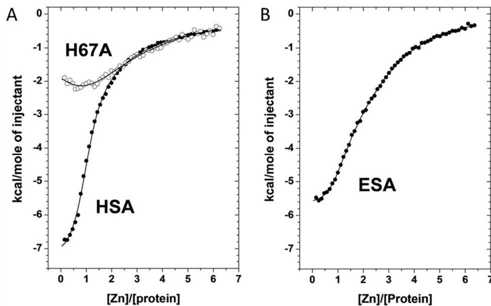
Measurement of \text{Zn}^{2+} binding affinity to HSA, H67A HSA mutant, and ESA by ITC. (A) ITC data for \text{Zn}^{2+} binding to HSA and the H67A mutant form. (B) ITC data for \text{Zn}^{2+} binding to ESA. In all cases the respective protein ( 50 \mu\text{M} ) was titrated with 5 \mu\text{l} injections of a 1.5 \text{ mM} \text{ZnCl}_2 solution for 55 injections.
