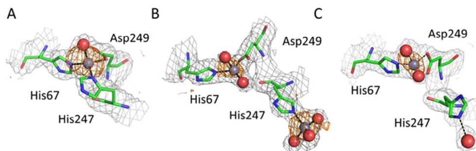
Representative structures showing dynamic behavior of His247 in ESA-Zn 2+ complexes. (A) ESA-Zn 2+ , 2.5 mM Zn 2+ , pH 7.4; 5IIH. (B) ESA-Zn 2+ , 30 mM Zn 2+ , pH 7.4; 5IJE. (C) ESA-Zn 2+ , 15 mM Zn 2+ , pH 6.5; 5IIX. Residues are shown in sticks representation, zinc ion in grey, oxygen in red, nitrogen in dark blue, carbon in green. Coordination bonds are marked with black dashed lines. Grey grid represents 2mF o - DF c map ( \sigma - 1.0), orange - anomalous map ( \sigma - 3.0).
