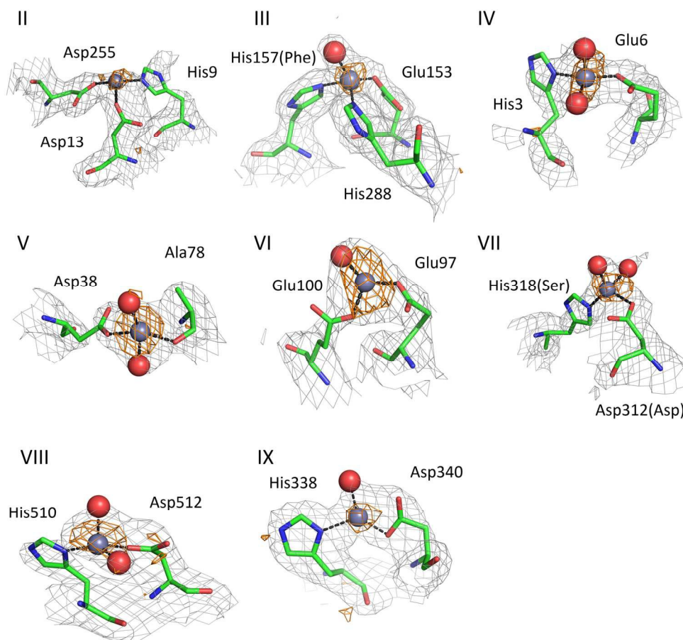
Secondary Zn^{2+} binding sites in the structures of ESA. Sites are numbered as in Table 3; only those coordinated by at least two protein residues are shown. Residues are shown in sticks representation, zinc ion in grey, oxygen in red, nitrogen in dark blue, carbon in green. Coordination bonds are marked with black dashed lines. Grey grid represents 2mF_o - DF_c map ( \sigma = 1.0 ), orange – anomalous map ( \sigma = 3.0 ). Residue numbers refer to HSA; in case of non-conserved residues, the HSA amino acid is given in parentheses.
