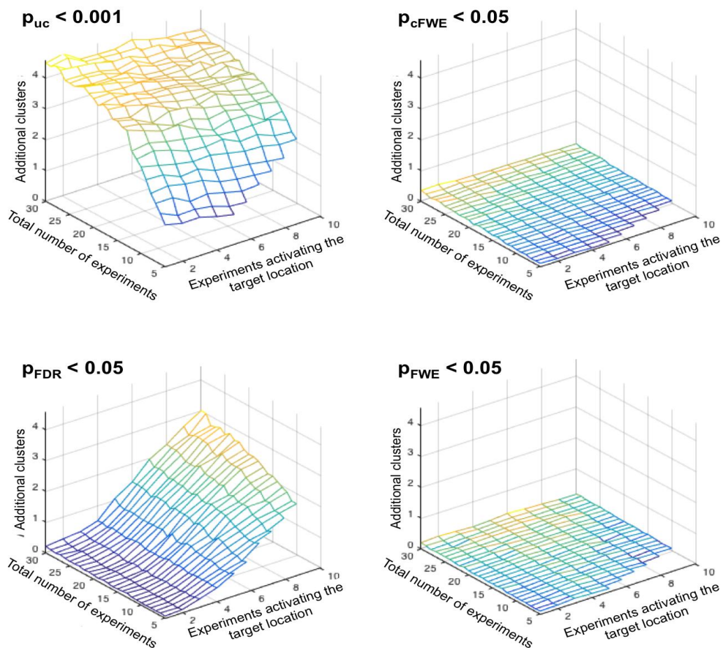
Figure 6: Average number of additional clusters of significant convergence outside of the “true”, i.e., target location in relationship to the total number of experiments, and the number of experiments activating the target location and the significance thresholding. Given that the distribution of the entire BrainMap database is known, these analyses allow quantifying deviations from the ground truth, similar to false positive findings. As can be seen, both voxel- and cluster-level FWE correction yield very low numbers of additional clusters. In turn, two interesting and orthogonal patterns may be noted for uncorrected thresholds and voxel-level FDR correction. When using the former ( p < 0.001 at the voxel level with k > 200\text{mm}^3 ) the number of additional clusters depends primarily on the total number of experiments entering the ALE. This may be expected because the chance for additional overlap increases if more experiments are present. For voxel-level FDR correction, however, the number of additional “false positive” clusters depends strongly on the number of experiments activating the
