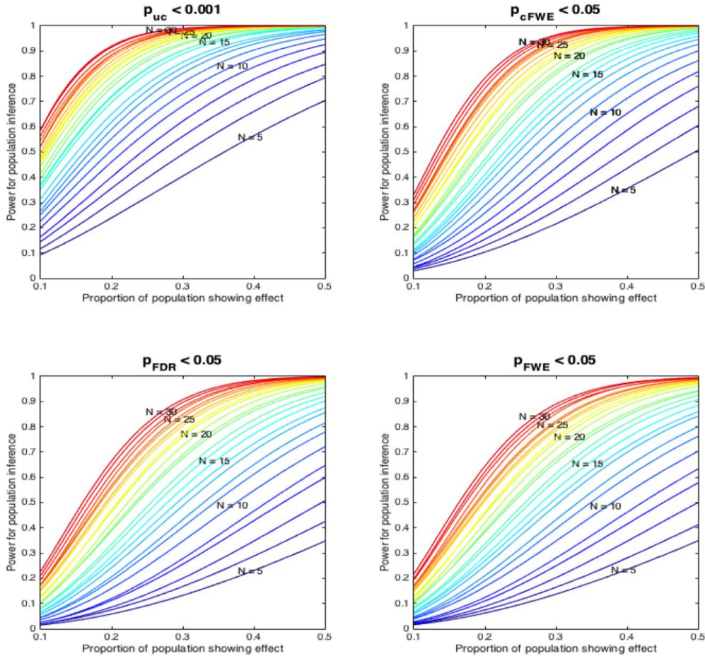
Figure 7: Power of inference on the underlying population of experiments assuming different “effect sizes” (proportion of the experiments in the underlying population showing an effect at a given location). The power to detect a given effect in the underlying population depends on the probability that x out of N experiments in an ALE analysis (assumed to be random samples from the underlying population) show the effect and the sensitivity of the ALE to identify it (cf. Figure 4). The total number of experiments in the respective simulated ALE is again coded in a spectral sequence. In spite of the differences in power between the thresholding methods, two trends are noticed. ALE analyses with less than 10-50 experiments yield a low power to find consistent effects. Even ALE analyses with 30 experiments are not very highly powered to reveal rare effects. In addition, we note that voxel-level FDR thresholding combines a low sensitivity (cf. Figure 4) with a high potential for false positive or spurious findings especially when there is a strong true effect (cf. figure 6).
