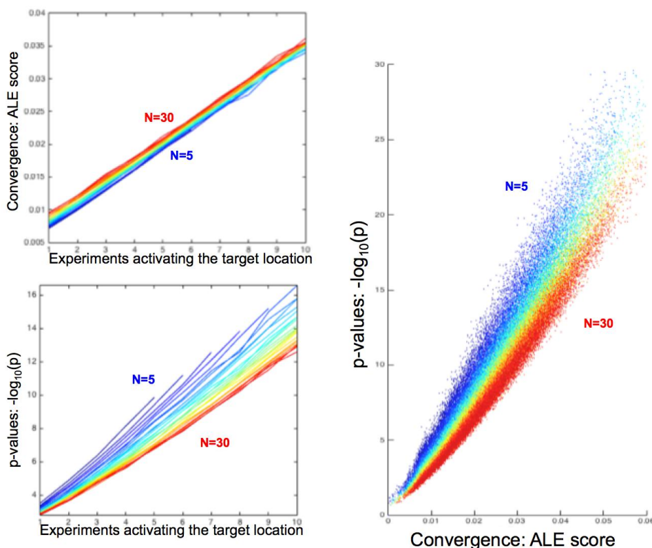
Figure 2: Characteristic behavior of the ALE scores and the corresponding p-values under the different simulation conditions as observed across 122,500 simulated ALE analyses. The total number of experiments in the respective simulated ALE is coded in a spectral sequence from 5 experiments (dark blue) to 30 experiments (dark red). The top left panel shows the average ALE-score (across simulations) at the simulated location (again using the highest local maximum within 4 voxels of the “true” location). ALE scores increase with number of experiments due to additional contribution of noise from other unrelated foci. The bottom left panel shows the average p-value (across simulations) at the simulated location (using the highest local maximum within 4 voxels of the “true” location). It shows that given the same number of experiments activating at a particular location, lower total numbers of experiments (i.e., greater prevalence of activated experiments) yield lower p-values. The right panel demonstrates the inverse relationships evident from the left panels by plotting ALE scores vs. p-values for the simulated location (again using the highest local maximum within 4 voxels of the “true” location) for all 122,500 simulations. Higher total numbers of experiments lead to higher p-values for the same ALE scores or, conversely, require higher ALE scores for the same p-value.
