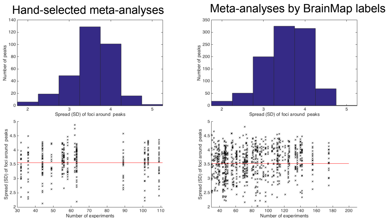
Figure 1: Evaluation of the activation spread to be used in the simulations. We assessed 15 hand-coded datasets for topic-based ALE meta-analyses (left side) as well as 105 datasets defined by combinations of the Behavioral Domain and Paradigm class meta-data from BrainMap (right side). After identifying the principal significant peaks in the ALE meta-analysis map, we computed the standard deviation of foci that contributed to that peak. In spite of the differences between both sets of meta-analyses with respect, they show homogeneity with the contributing experiments with a similar concentration (3-4 mm standard deviation) in each case (upper panels). Importantly, this spread seems independent of the number of experiments that constitute the respective meta-analyses (lower panels). Based on these data, the 500 simulations used spreads of 2 mm (50 times), 3 mm (200 times), 4 mm (200 times) and 5 mm (50 times) around the true location of the simulated effect.
