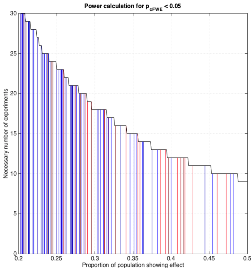
Figure 9: Illustration of “effect sizes” (proportion of the experiments in the underlying population showing an effect at a given location) found for real-life ALE analyses. Here we used the same datasets as in Figure 1 and combined them with the sample-size calculations for cluster-level FWE inference. Red lines correspond to peaks from the hand-coded datasets for topic-based ALE meta-analyses and blue lines to the datasets defined by combinations of the Behavioral Domain and Paradigm class meta-data in BrainMap. Note that strong effects such as 40% or more of a dataset showing a particular effect are rare, while “effect sizes” of 0.2 - 0.25 are much more common.
