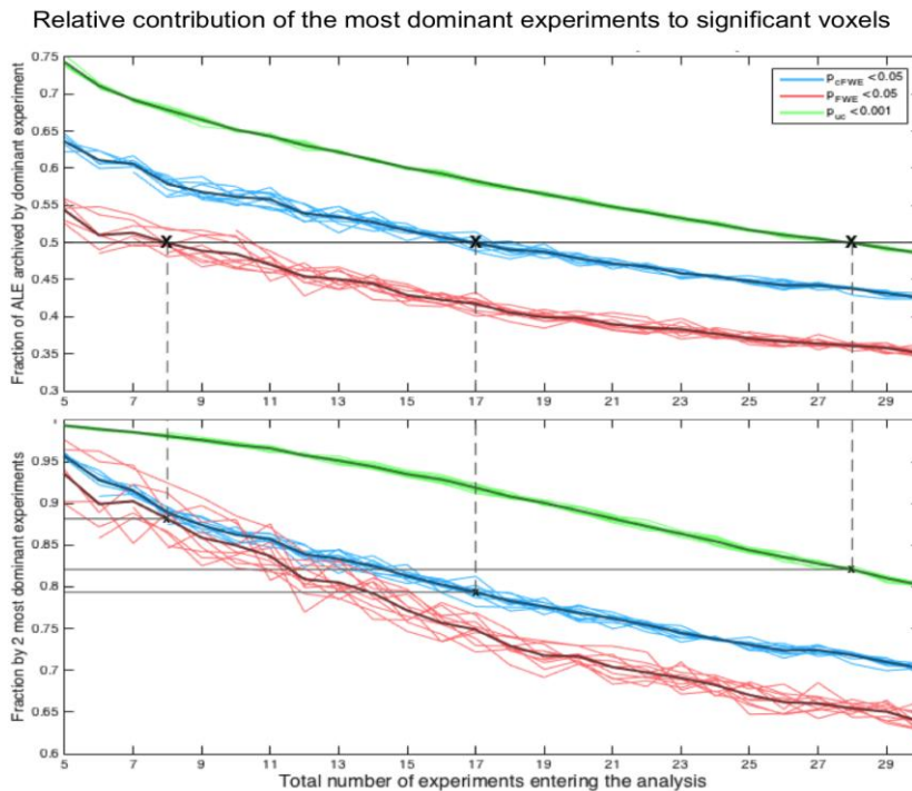
Figure 3: To quantify the empirical observation that significant effects may be largely driven by a single experiment if the total number of experiments is relatively low and hence to provide quantitative guidelines on the minimal number of experiments needed for valid ALE analyses, we quantified the number of experiments contributing to the significant clusters under different thresholding methods. This analysis is not based on the “true” location of the effect but rather on those at which random convergence happened through the structure of the BrainMap database. For each of these additional clusters, surviving statistical thresholding, we computed the fraction of the ALE value that was accounted for by the most dominant (top panel) and two most dominant (lower
