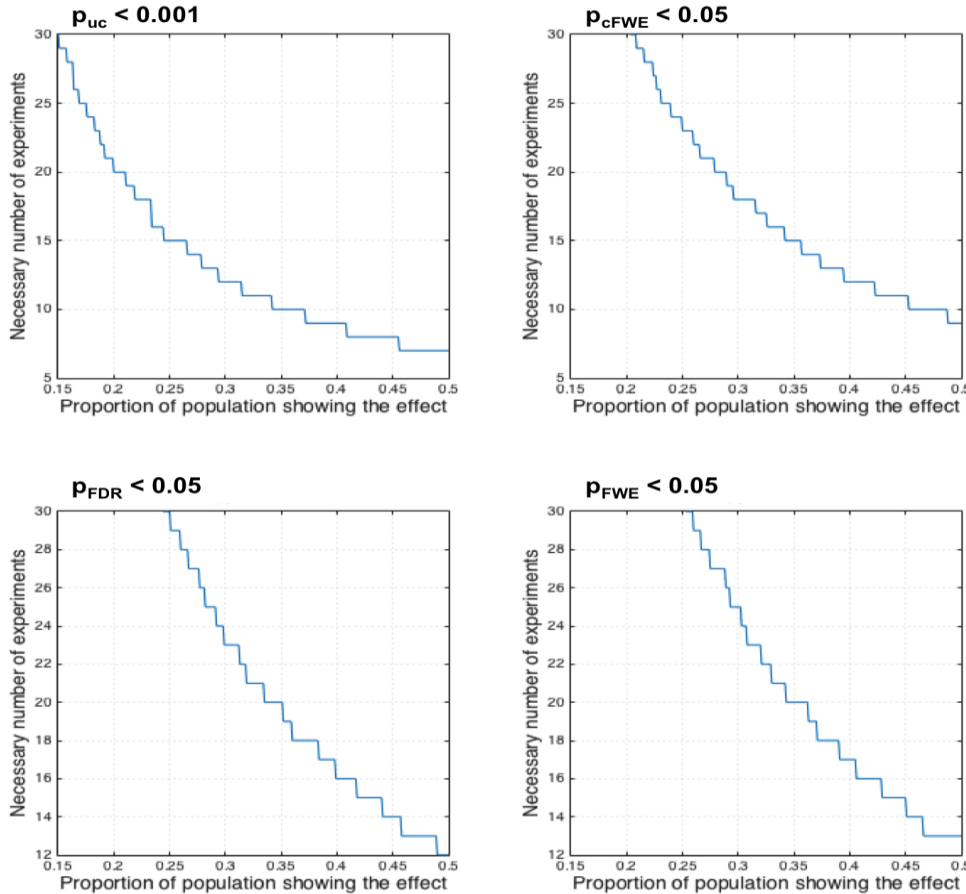
Figure 8: Sample size calculations for ALE meta-analyses assuming a desired power of 80% given different “effect sizes” (proportion of the experiments in the underlying population showing an effect at a given location) for each of the four assessed thresholding approaches.
