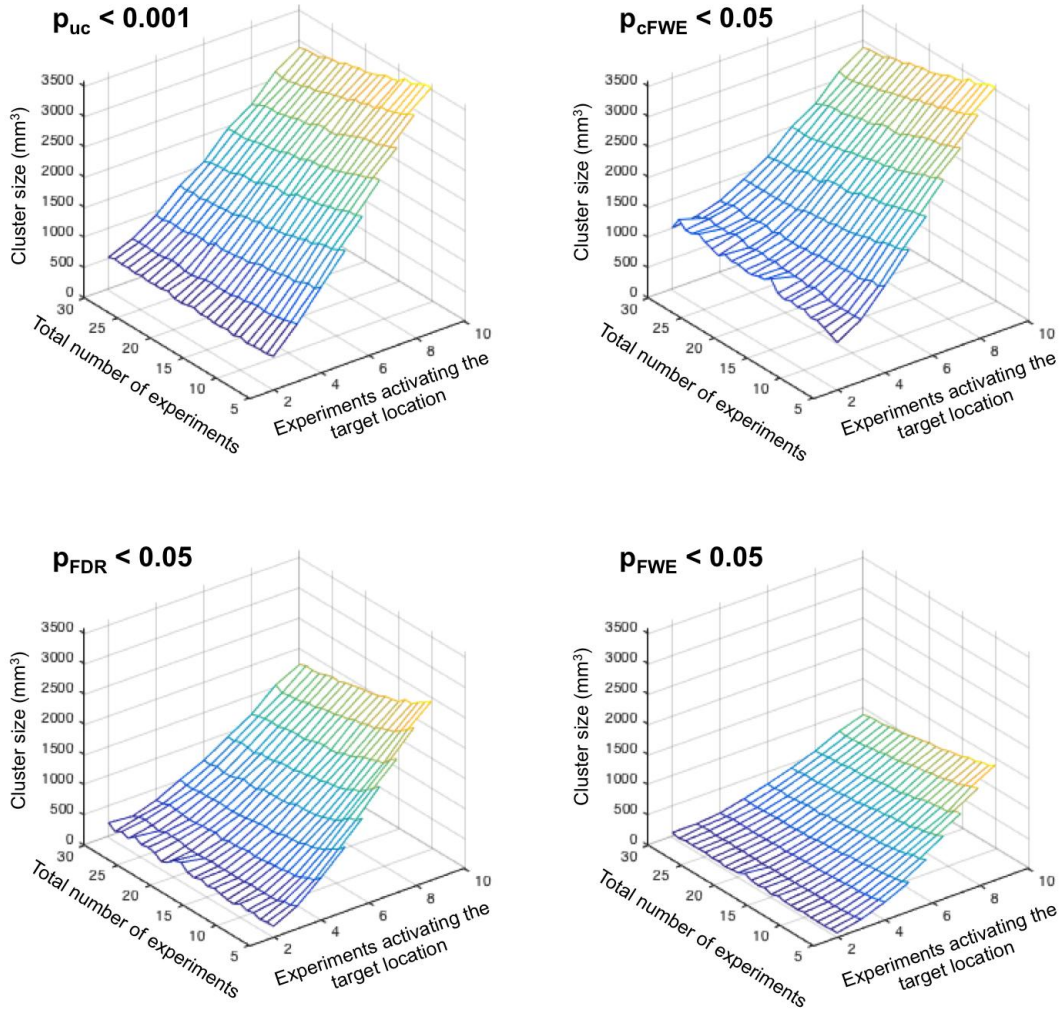
Figure 5: Cluster-size of the super-threshold cluster at the “true” location, i.e., the target of the simulation, in relationship to the total number of experiments and the number of experiments activating the target location. It becomes apparent that the cluster size increases strongly with the number of experiments activating the “true” location. In turn, clusters become smaller when the total number of experiments increases given the same number of experiments activating the target location. Finally, we note that FDR and in particular voxel-level FWE thresholding yields much smaller clusters than cluster-level FWE thresholding.
