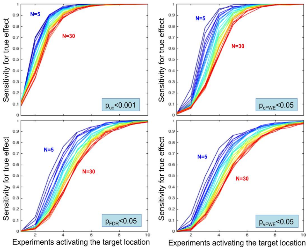
Figure 4: Sensitivity of ALE to detect the simulated true convergence given the number of experiments activating the target location. The total number of experiments in the respective analyses is coded in a spectral sequence from 5 experiments (dark blue) to 30 experiments (dark red). Three key aspects may be noted. First, a higher total number of experiments leads to a right-shift in the sensitivity curves. Second, independent of the
