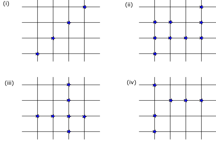
FIGURE 2. In (ii) and (iii), \Gamma is connected. The subsets in (i), (iv) are not connected; the subset in (i) has four components and that in (iv) has three.
