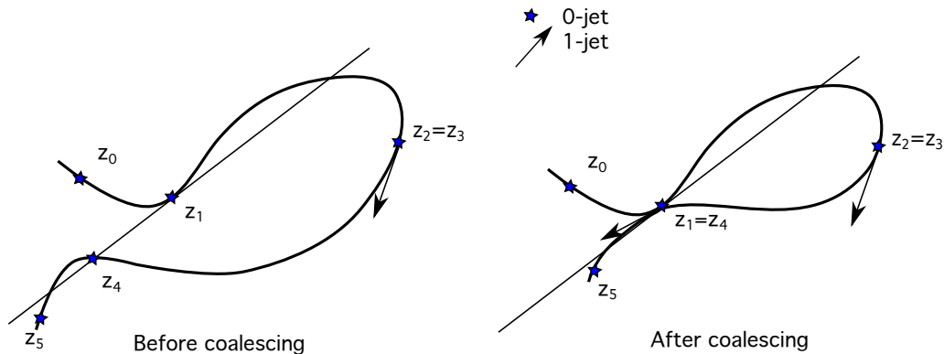
FIGURE 10. Coalescence of distinguished points in a pointed curve does not require the points to be adjacent, in some sense, on the curve. Here the coalescence takes place along the straight line. Note there needs to be a well defined tangent of C at the point of coalescence.
