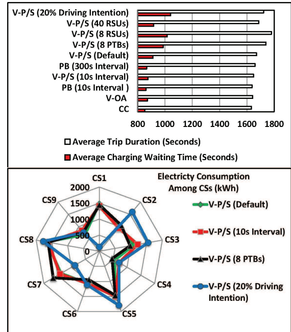
Fig. 5. Charging Performance
