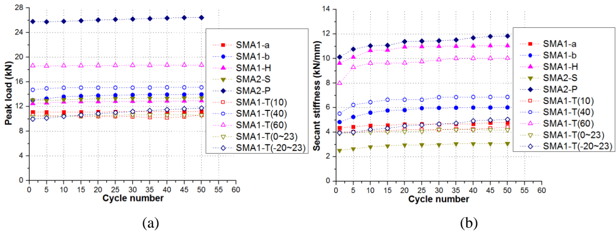
Fig. 5 Strength and stiffness responses of SMA washer specimens
