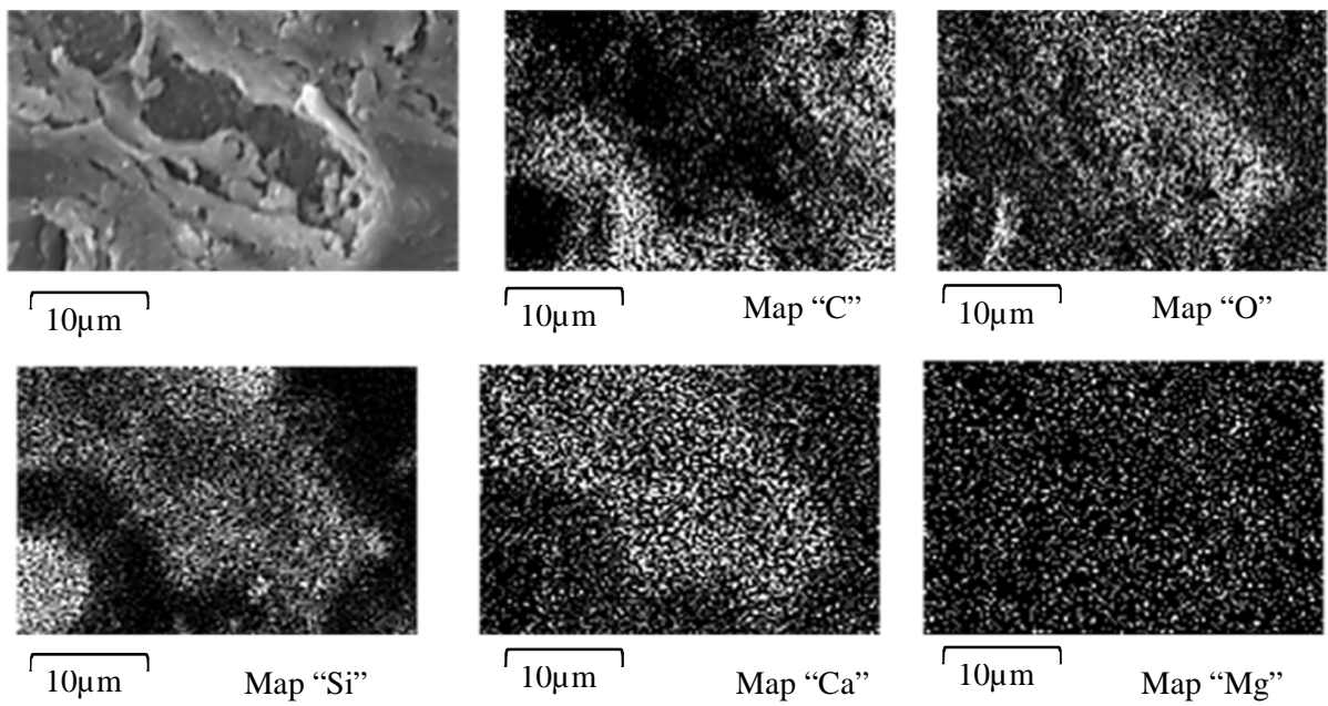
Figure 9 Elemental analysis of a section of Limeboo DL85-S2 pre-treated with a saturated solution of \text{Ca(OH)}_2 . a) SEM image. b) to g) EDX maps of carbon, oxygen, silicon, calcium and magnesium in the same imaged section.
