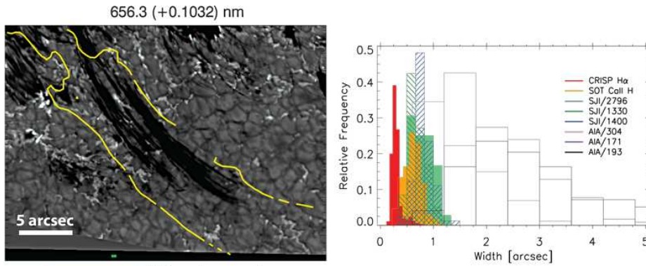
Fig. 19 Left: A high-resolution (super-resolution) image of a post-flare loop taken with the CRisp Spectro-Polarimeter (CRISP) at the Swedish 1-m Solar Telescope (SST) in the H\alpha far red-wing (656.3 nm +0.1032 nm) (Scullion et al. 2014). The appearance of coronal rain (dark strands in H\alpha ) is co-spatial with high temperature emission in the SDO/AIA 17.1 nm channel (yellow contours, \log T = 5.8 ) from the coronal loop. Right: Histogram of coronal rain widths for two datasets combining various wavelengths: H\alpha with the SST (in red, average measured logarithmic temperature \log T \approx 3.8 ), Ca II H with Hinode/SOT (orange, \log T \approx 4 ), Mg II k 279.6 nm with IRIS/SJI (light green, \log T \approx 4.2 ), C II 133.0 nm with IRIS/SJI (dark green, \log T \approx 4.3 ), Si IV 140.0 nm with IRIS/SJI (blue, \log T \approx 4.8 ), He II 30.4 nm with SDO/AIA (light purple, \log T \approx 5 ), Fe IX 171 with SDO/AIA (dark purple, \log T \approx 5.9 ), and Fe XII 19.3 nm with SDO/AIA (black, \log T \approx 6.2 ). Explanation for these datasets can be found in Antolin et al. (2015b). The bin size in each wavelength is set to the spatial resolution of each instrument. Strand-like structure in these loops extends from chromospheric to at least transition region temperatures. The shape of the distributions strongly suggest that the bulk of the coronal rain widths remains undetected at present day resolution. Also compare to the statistical analysis of strands in this coronal loop by Scullion et al. (2014).
