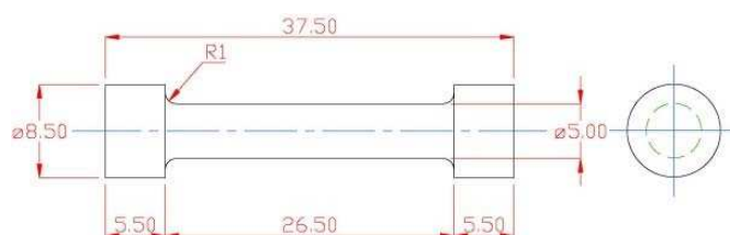
Figure 7 – Tensile test specimen dimensions (dimensions in mm)
