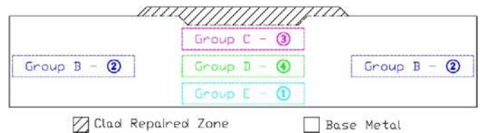
Figure 10 – Group B to E Tensile test result ranking
