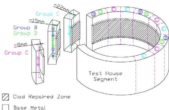
Figure 6 – Extraction locations of Group B to E specimens
