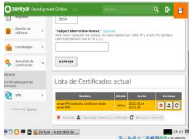
Figura 84: VPN
