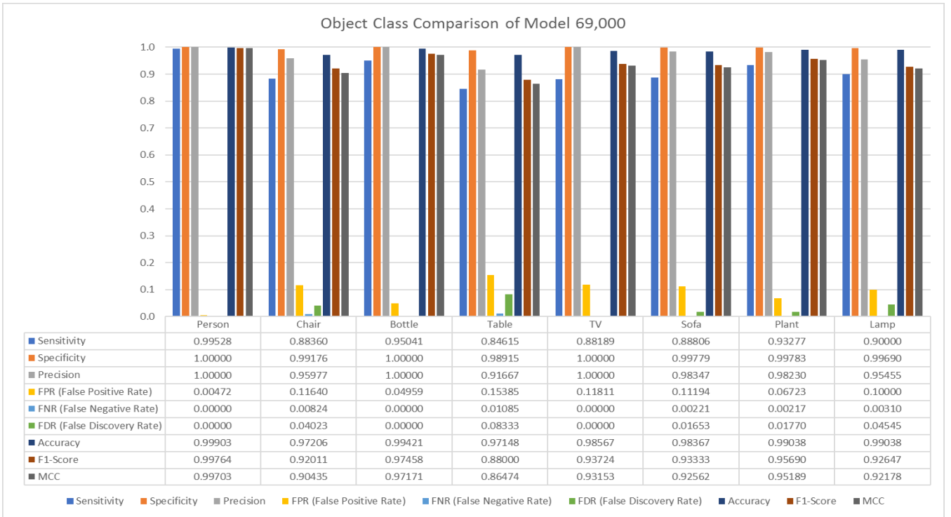
Fig.2. Detection of common objects in a smart home.
