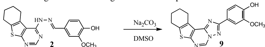
Scheme 3. Oxidative cyclisation and rearrangement of Exo2 with sodium carbonate
