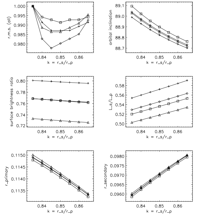
Fig. 12. EBOP solutions for VZ Hya for a range of fixed k values. Linear limb-darkening coefficients by van Hamme (1993) were adopted. The upper left panel shows normalized rms errors of the fit to the observations. Symbols are: cross y ; diamond b ; triangle v ; square u .
