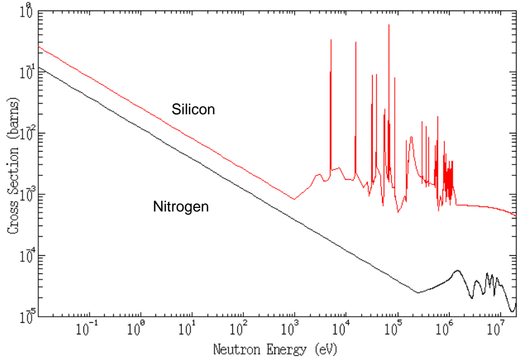
Figure 6.6: Variation of radiative capture cross section of Si and N with neutron energy From the on-line interactive spectrum facility at http://hpngp01.kaeri.re.kr/CoN/endlplot.shtml [Cha]
