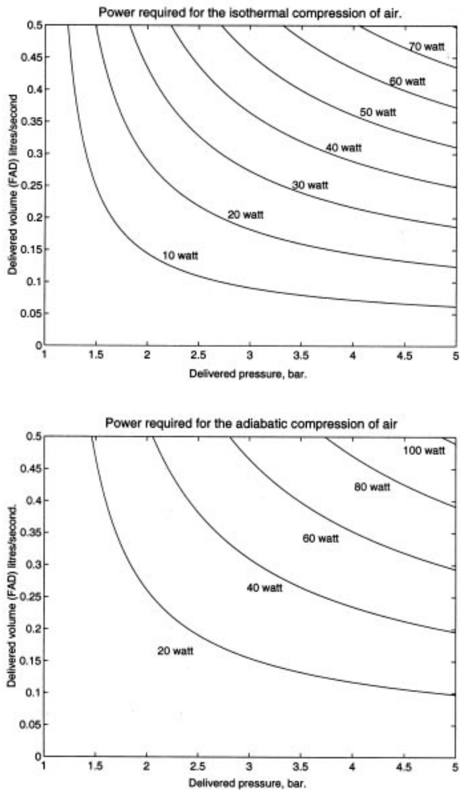
Figure 5.20: Contour plots of power required to compress air isothermally and adiabatically. Note: Pressure values are absolute and not gauge pressures.
