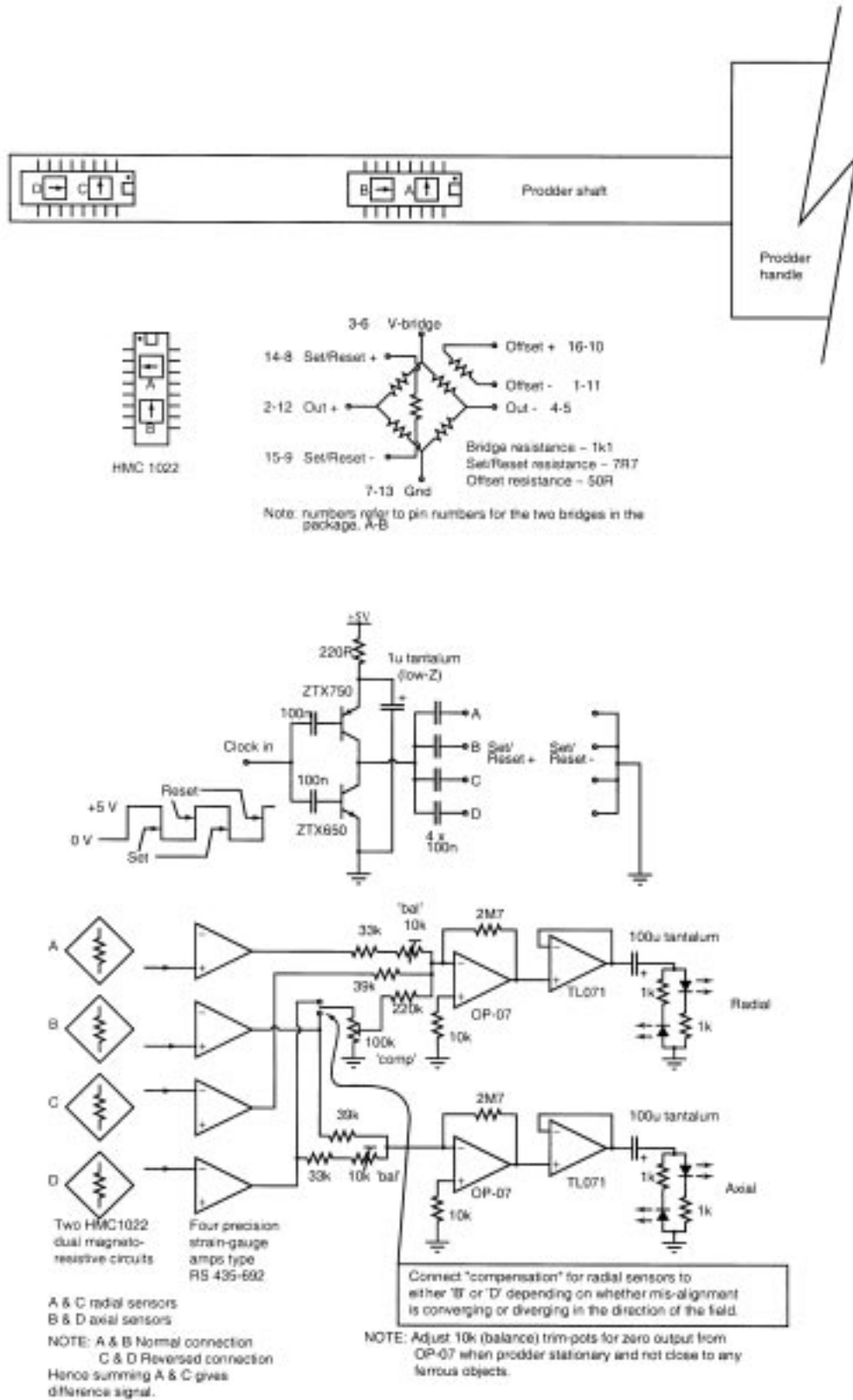
Figure 5.5: Differential magnetometer prodder circuit diagram.
