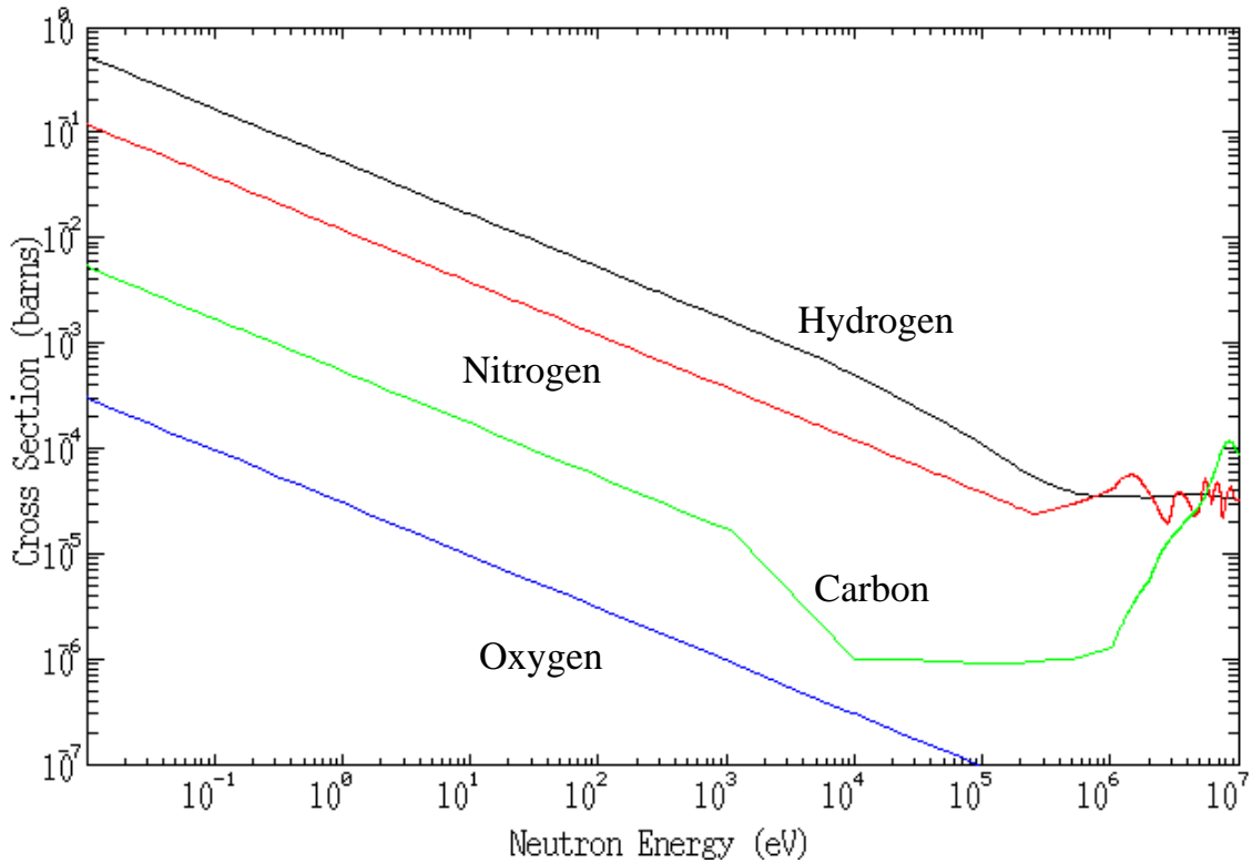
Figure B.1: Neutron-gamma capture cross sections for constituent elements of explosives. From the on-line interactive spectrum facility http://hpngp01.kaeri.re.kr/CoN/endfplot.shtml [Cha].
