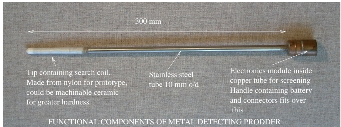
Figure 5.2: Metal detector prodder.
