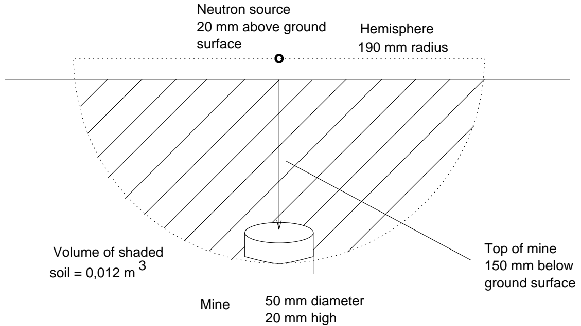
Figure 6.5: Diagram to illustrate calculation of order of magnitude of nitrogen background. The nitrogen in the soil nearest the neutron source receives a greater neutron flux density than the mine due to both the inverse square reduction in flux with distance from the source and to the thermalisation of neutrons and their subsequent capture which is dominated by soil moisture (see section 6.7.2 above).
