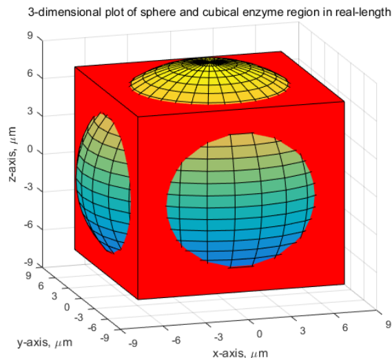
Figure 15. Plot of the spherical and cubical enzyme region shapes with the same volume for small r_{\text{enz}} case.
