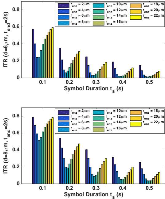
Figure 11. ITR of ST-ARx with varying r_{enz} and t_s for d = 6 \mu\text{m} (Top) and 8 \mu\text{m} (Bottom) ( r_r = 5 \mu\text{m} , t_{end} = 2.0 \text{ s} , \Lambda_{1/2}^{1 \mu\text{m}} = 0.002 \text{ s} ).
