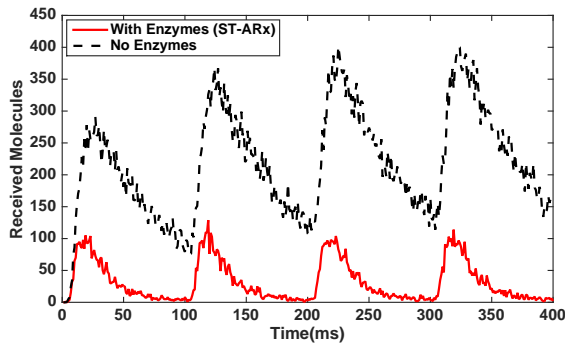
Figure 5. Received signals for ST-ARx system for four symbol periods when t_s = 0.1 s. ( d = 4 \mu\text{m} , r_r = 5 \mu\text{m} , r_{enz} = 8 \mu\text{m} , t_{end} = 0.4 s, \Lambda_{1/2}^{1 \mu\text{m}} = 0.002 s).
