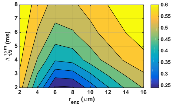
Figure 13. Heatmap of ITR with varying r_{enz} and \Lambda_{1/2}^{1 \mu\text{m}} for ST-ARx scenario ( d = 6 \mu\text{m} , r_r = 5 \mu\text{m} , t_s = 0.1 \text{ s} , t_{end} = 2.0 \text{ s} ).
