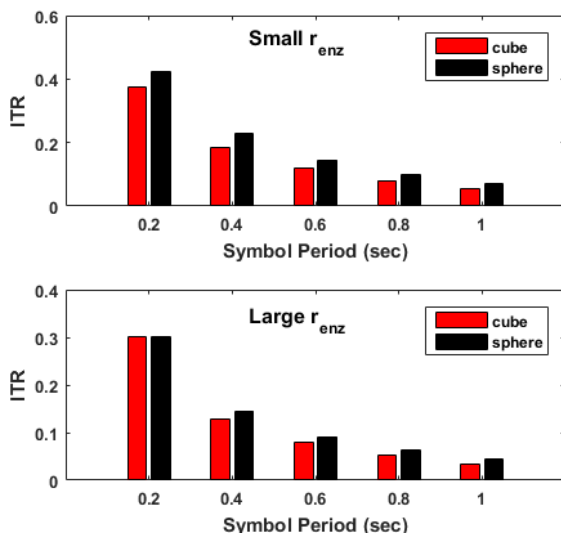
Figure 14. ITR of ST-ARx for sphere and cube enzyme regions of different size ( d = 8 \mu\text{m} , r_r = 5 \mu\text{m} , t_{\text{end}} = 2.0 \text{ s} , \Lambda_{1/2}^{1\mu\text{m}} = 0.002 \text{ s} ).
