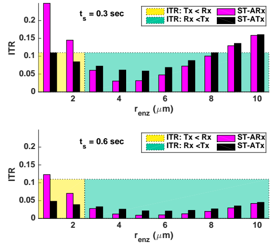
Figure 10. ITR of ST-ARx, and ST-ATx scenarios for t_s = 0.3 \text{ sec} (Top) and 0.6 \text{ sec} (Bottom) and different r_{\text{enz}} ( d = 4 \mu\text{m} , 8 \mu\text{m} , r_r = 5 \mu\text{m} , t_{\text{end}} = 2.0 \text{ s} , \Lambda_{1/2}^{1\mu\text{m}} = 0.002 \text{ s} ).
