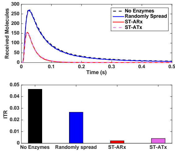
Figure 8. Received signals (Top) and ITR (Bottom) for comparing deployment schemes ( d = 4 \mu\text{m} , r_r = 5 \mu\text{m} , r_{\text{enz}} = 6 \mu\text{m} , t_s = 1.0 \text{ s} , t_{\text{end}} = 2.0 \text{ s} , \Lambda_{1/2}^{1\mu\text{m}} = 0.002 \text{ s} ).
