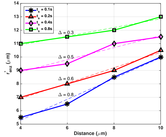
Figure 12. r_{enz}^* depending on the distance for different t_s for ST-ARx scenario with fitting lines ( r_r = 5 \mu\text{m} , t_{end} = 2.0 \text{ s} , \Lambda_{1/2}^{1 \mu\text{m}} = 0.002 \text{ s} ).
