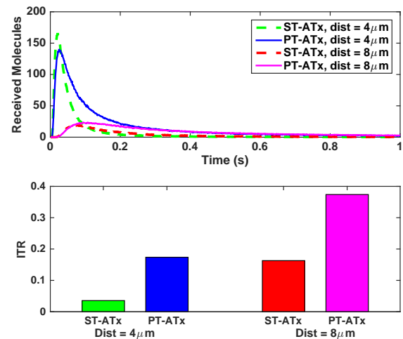
Figure 7. Received signals (Top) and ITR (Bottom) for comparing sphere and point source scenarios ( r_r = 5 \mu\text{m} , r_{enz} = 2 \mu\text{m} , t_s = 0.5 s, t_{end} = 2.0 s, \Lambda_{1/2}^{1 \mu\text{m}} = 0.002 s).
