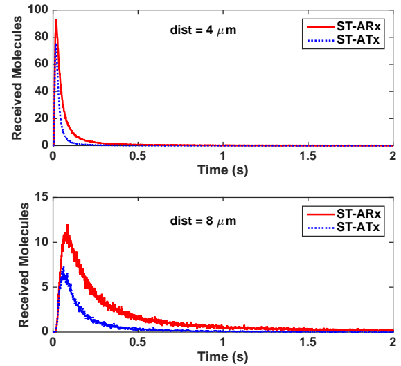
Figure 9. Received signals of ST-ARx, and ST-ATx scenarios for d = 4 \mu\text{m} (Top) and 8 \mu\text{m} (Bottom) ( r_r = 5 \mu\text{m} , r_{\text{enz}} = 2 \mu\text{m} , t_{\text{end}} = 2.0 \text{ s} , \Lambda_{1/2}^{1\mu\text{m}} = 0.002 \text{ s} ).
