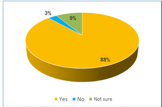
Fig. 4: M-learning usage
