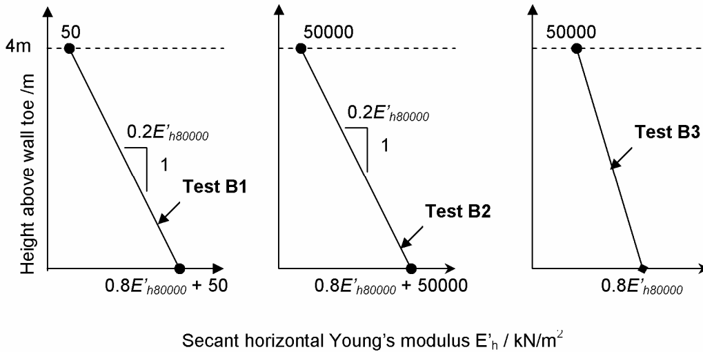
Figure 5. Profiles of Young's modulus with depth used in the test series B.
