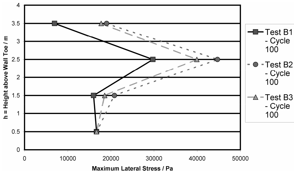
Figure 7. Lateral Stress after 100 cycles against Height Comparison for different Young's modulus Profiles.
