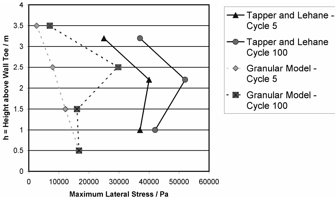
Figure 6. Lateral Stress against Height Comparison of Granular Model Prediction against experimental data of Tapper & Lehane (2004).
