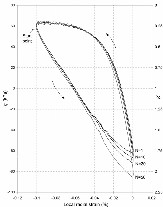
Figure 1. Typical Curve of Deviator Stress and Earth Pressure Coefficient K against Local Radial Strain for Leighton Buzzard Sand by Xu (2005).
