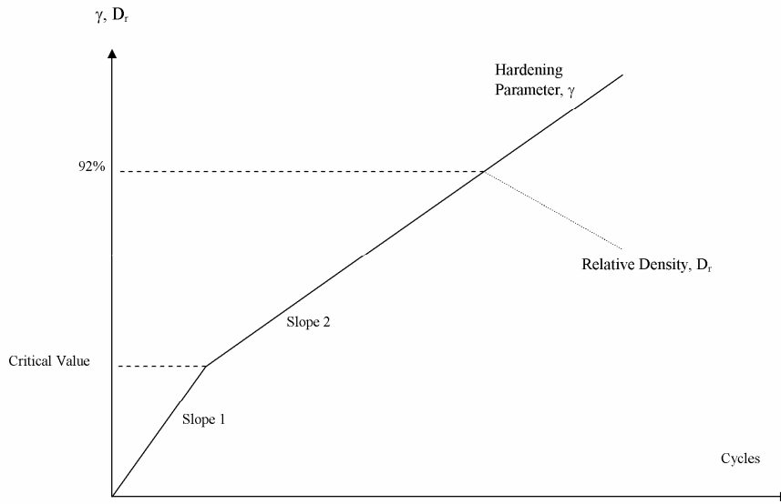
Figure 2. Development of the Hardening Parameter, \gamma , against cycles of Radial Strain.
