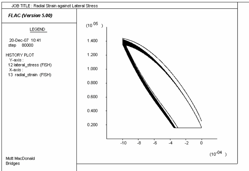
Figure 3. Typical Curve of Lateral Stress against Radial Strain from FLAC analysis of the triaxial test using the granular constitutive model.
