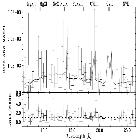
Fig. 8. The RGS spectra (RGS1 in black and RGS2 in gray), along with Model A, derived from the EPIC spectral analysis. The positions of lines expected to be strong are also reported. The ratio between model and observed spectra is shown in the lower panel.
