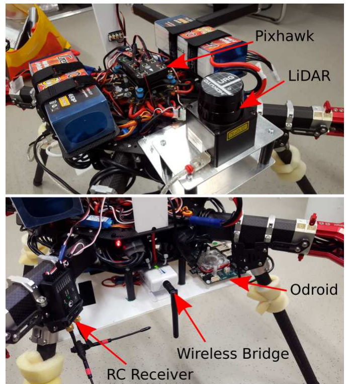
Fig. 3. Major system components onboard octocopter vehicle
