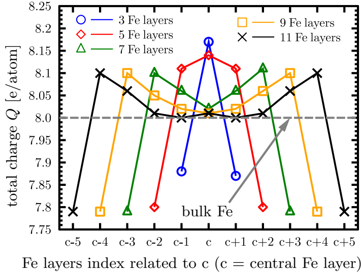
Figure 6. (Color online) Net charge for different Fe thicknesses compared to the bulk Fe value of 8e/\text{atom} . The values have been shifted to the centre of the Fe slice. The lines are guides for the eye.
