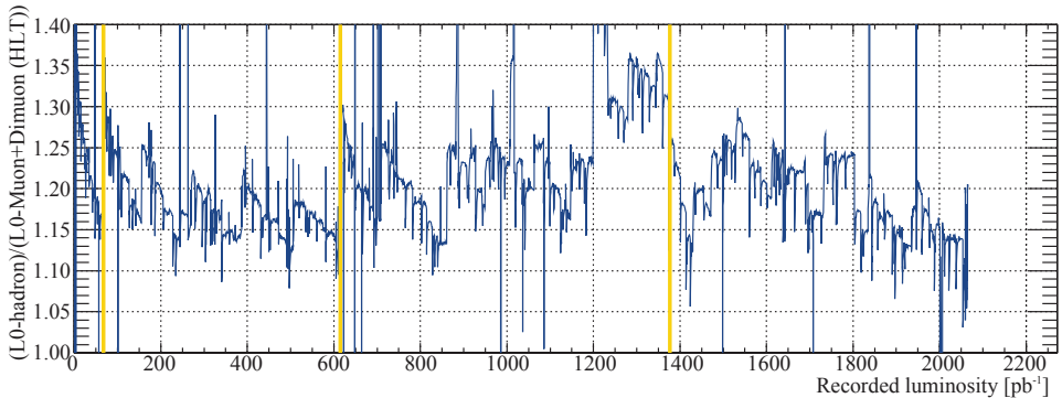
Fig. 29. Ratio between the rate of events triggered by the L0-hadron trigger, based on the HCAL, and Muon-based triggers. Distinct increases in rate, e.g. as at a recorded luminosity of around 50 \text{ pb}^{-1} , correspond to the application of a new set of PMT gains.
