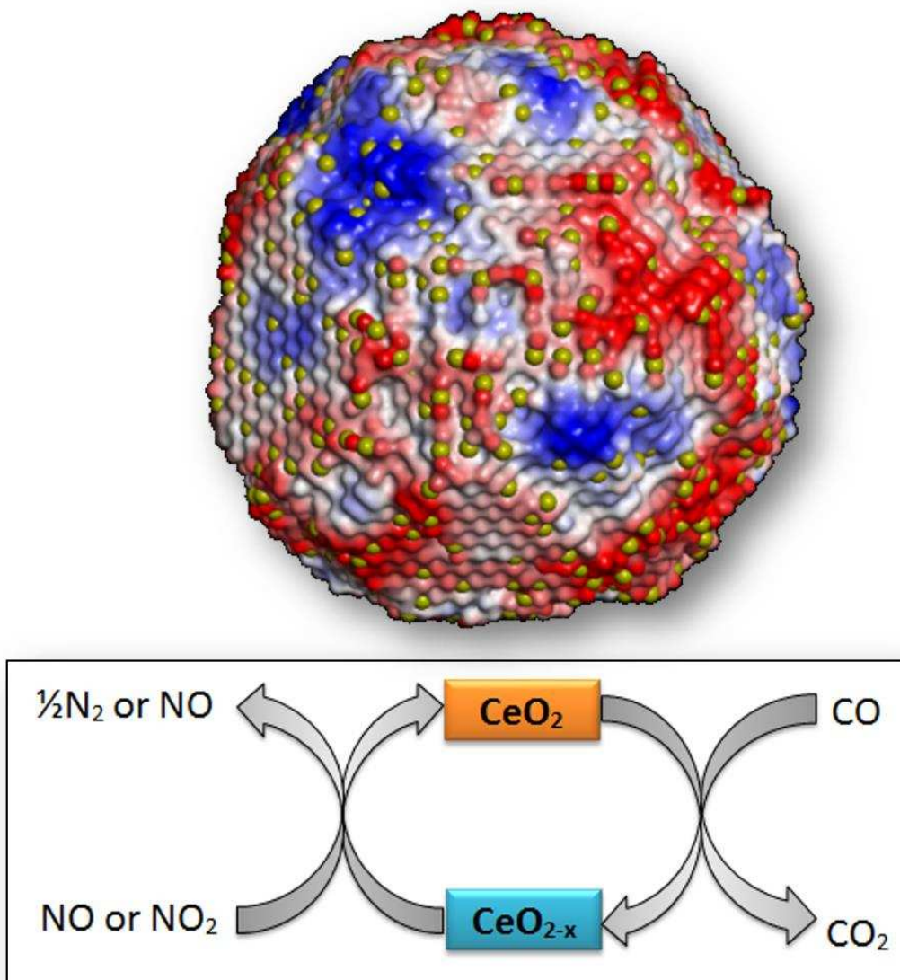
Figure 1 Schematic, illustrating the oxidation of \text{CO} to \text{CO}_2 ( \text{CeO}_2 reduces to \text{CeO}_{2-x} ) and reduction of \text{NO}_2 to \text{NO} ( \text{CeO}_{2-x} oxidises to \text{CeO}_2 ). The top image shows a model ceria nanoparticle coloured according to how (energetically) facile it is to extract surface oxygen (red–white–blue: easy to difficult to extract). The yellow dots indicate the positions of \text{Ce}^{3+} ions.
