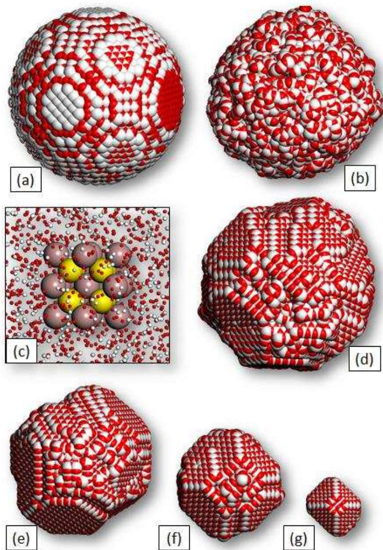
Figure 3 Atomistic models of polyhedral ceria nanoparticles. (a) Sphere cleaved from parent bulk material, (b) structure of the molten nanoparticle, (c) structure of the crystalline seed at the centre of the nanoparticle, (d) final, low-temperature structure of the crystalline nanoparticle, (d), (e), (f) and (g) are drawn to scale and represent the final structures of the 9, 8, 6 and 3.5 nm nanoparticles respectively. Cerium is coloured white and oxygen is red.
