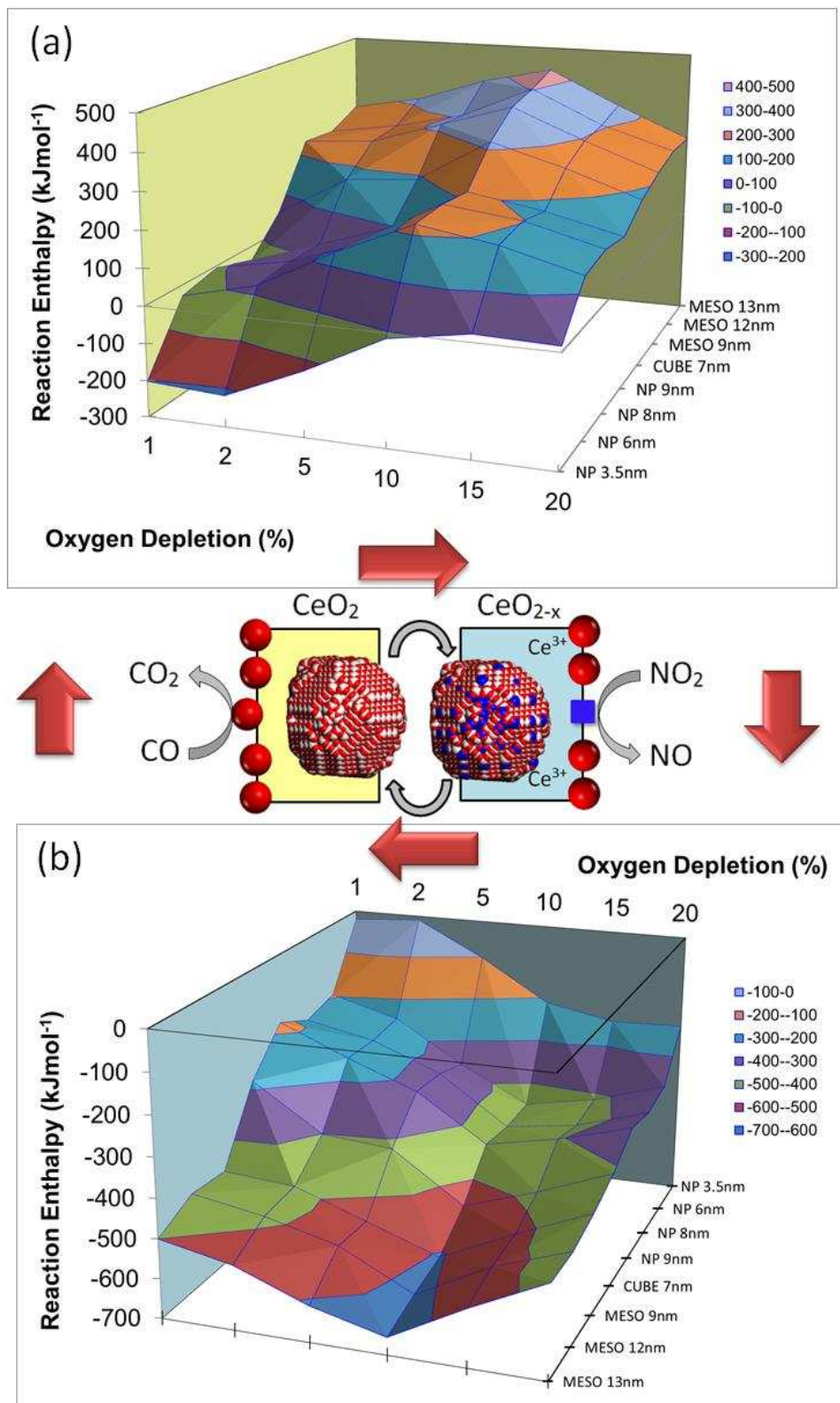
Figure 7 Activity map for nanoceria as a function of defect content, nanoarchitecture and size. Activity toward (a) CO oxidation (b) \text{NO}_2 reduction. The schematic at the centre illustrates the catalytic cycle.
