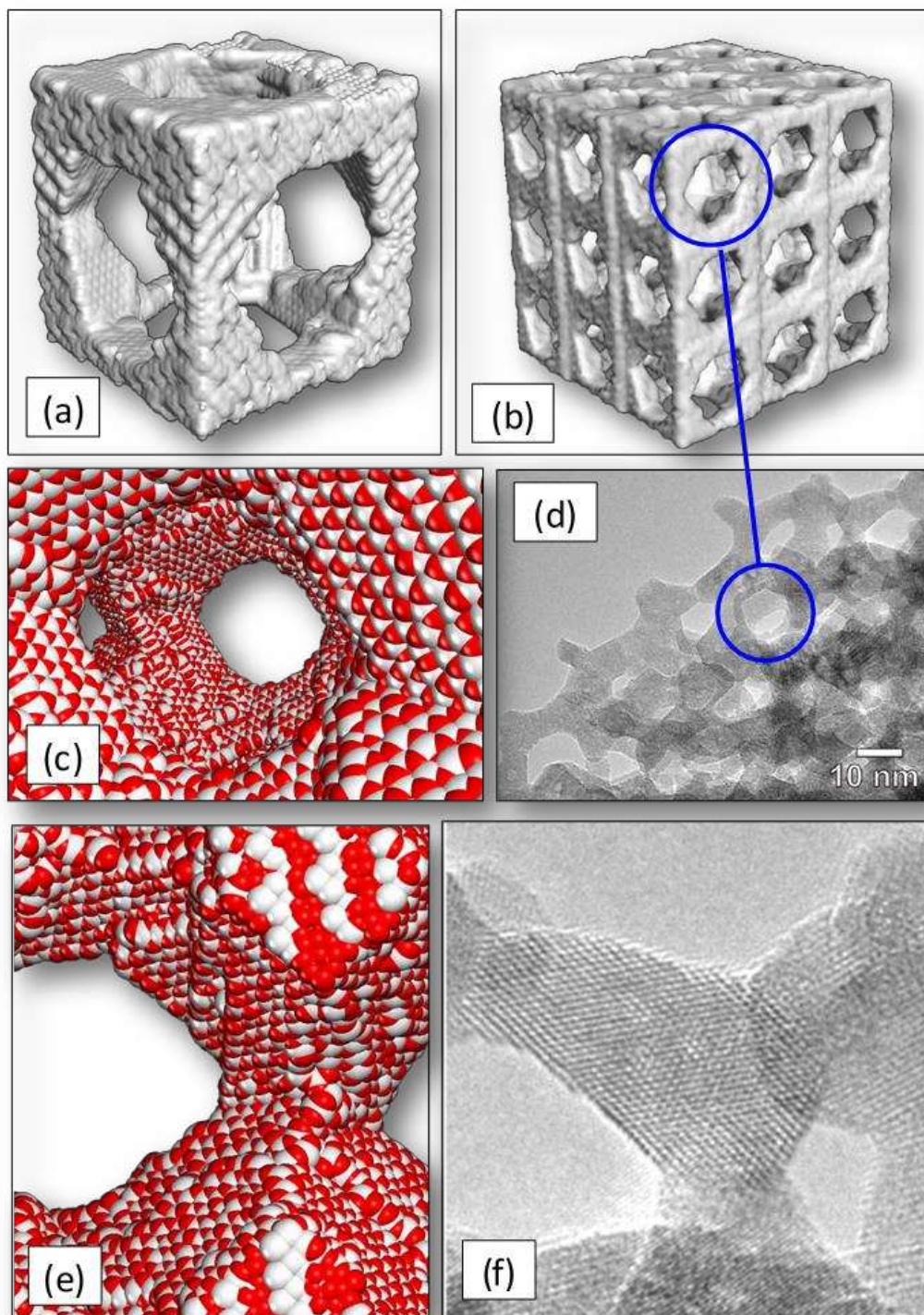
Figure 4 Atom-level models of mesoporous \text{CeO}_2 compared to the real material. (a) Unit cell of mesoporous ceria (model), (b) supercell comprising 9 unit cells to show the connectivity of pores. (c) model structure of an internal pore, (d) HRTEM of real mesoporous \text{CeO}_2 , (e) atomistic model of a pillar comprising the pore wall, (f) HRTEM of the real material. (d) and (e) are taken with permission from ref [26]. Copyright American Chemical Society. Cerium is coloured white and oxygen is red. All images
