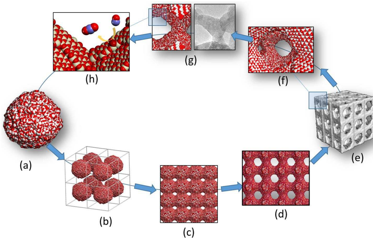
Figure 2 Strategy used to generate atom-level models of mesoporous ceria. (a) amorphous \text{CeO}_2 nanobuilding block. (b) building blocks introduced into simulation cell. (c) 'self-assembly' of nanobuilding blocks into mesoporous architecture. (d) crystallisation of system (evolution of fluorite crystal structure, grain-boundaries and dislocations). (e) Three-dimensional Connolly surface of atom positions in (d). (f) view showing the pore structure. (g) structural accord with experiment (HRTEM). (h) Oxidation of CO to \text{CO}_2 using oxygen from ceria catalyst. The images all reflect simulated atom positions; none are schematic.
