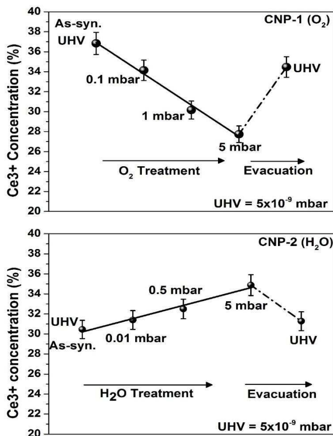
Figure 8 Percentage of Ce^{3+} calculated from integrated area of Ce3d spectrum, fig S11, S12, as a function of O_2 (top) and H_2O (bottom) gas pressure for CNP-1 and CNP-2.
