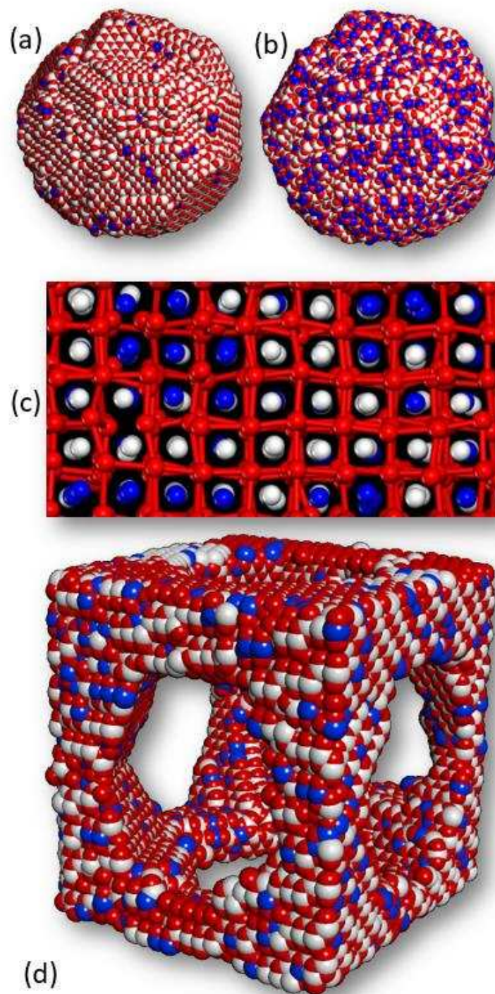
Figure 5 Models of reduced ceria nanostructures. (a) 13 nm polyhedral nanoparticle with 1% oxygen depletion. (b) 13 nm nanoparticle with 10% oxygen depletion. (c) Segment cut through (b) showing the oxygen sublattice disorder. (d) mesoporous ceria model with 5% oxygen depletion. Ce 4+ is coloured white, Ce 3+ is coloured blue and oxygen is red.
