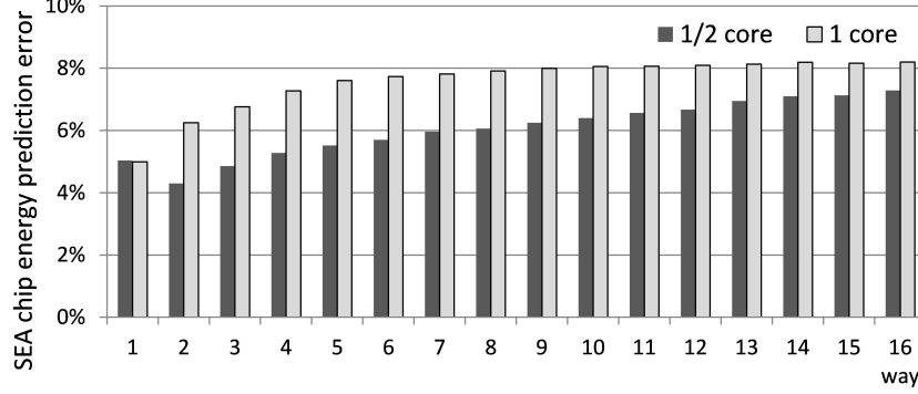
Fig. 6. SEA_{chip} prediction error for a 4 SMT core setup and 16-way LLC
