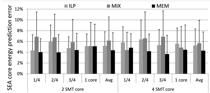
Fig. 5. SEA_{core} prediction error, under 2, 4 SMT cores setup, using I, X, M types workloads
