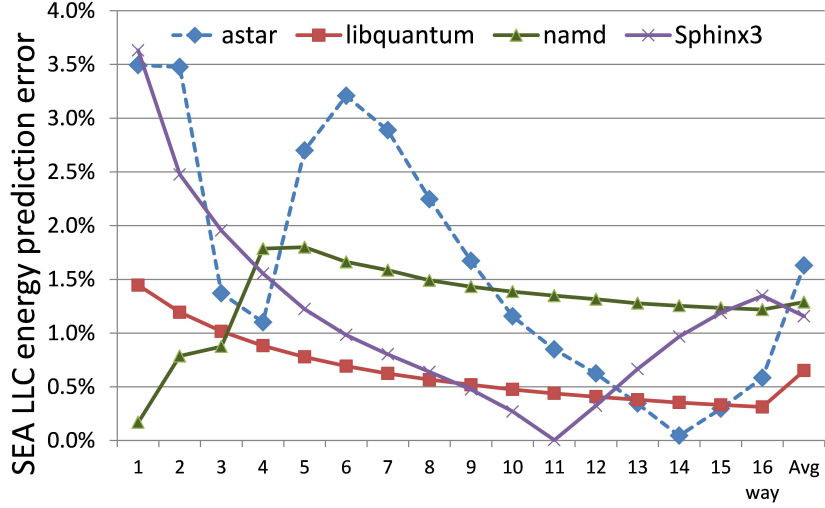
Fig. 2. SEA_{LLC} prediction error for a workload consisting of benchmarks astar , libquantum , namd , and sphinx3 in a 16-way associative LLC
