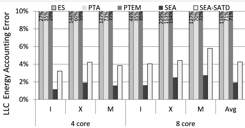
Fig. 3. LLC energy accounting error, under CMP 4, 8 cores setup, using I, X, M types workloads
