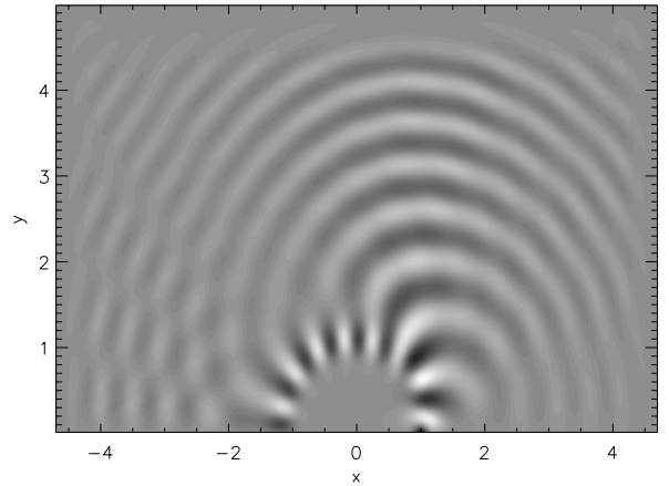
Fig. 3. Contours of V_{\text{perp}} for a driver period of 0.48 at the termination of driving ( t = 144 ). The driver has excited a dominant eigenmode with a period of 0.51. Note that the pattern is highly asymmetric due to the footpoint driver. The mode number for this eigenmode is n = 16 .
