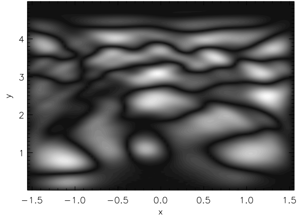
Fig. 11. Pattern of |V_{\text{perp}}| across the box for nearby reflecting boundary conditions, using the same physical parameters as used in the main simulations. The mode number is 5, and the driver period is 1.32, the observed period is 1.52.
