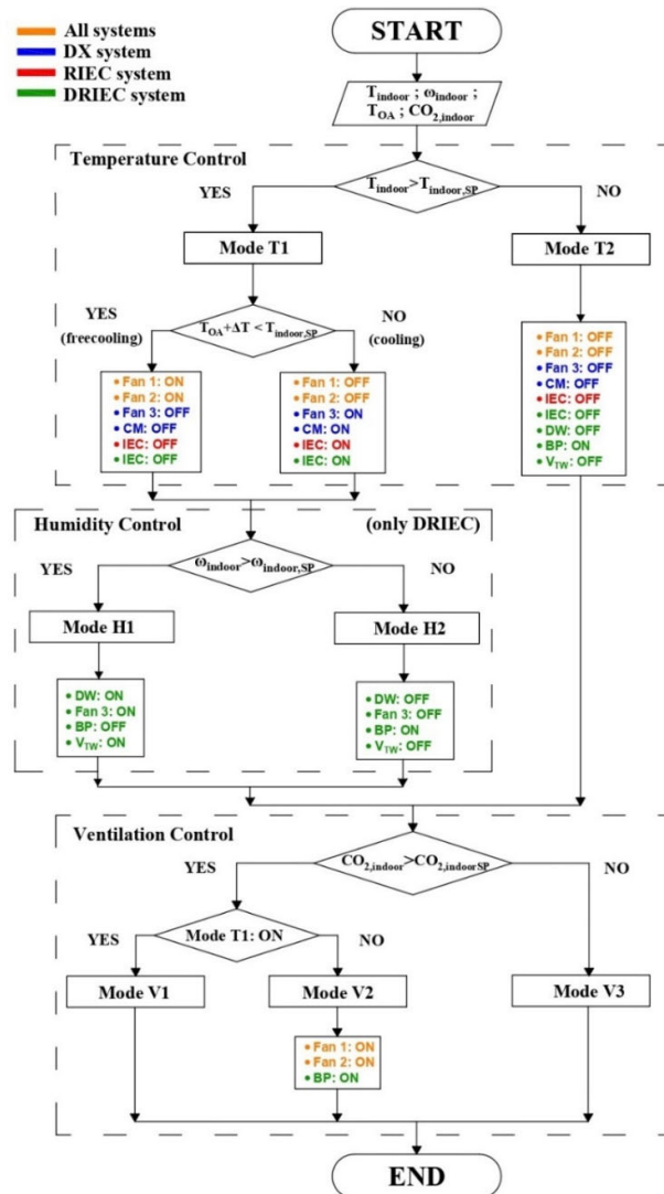
Figure 4. Air-cooling systems control logic diagram.
