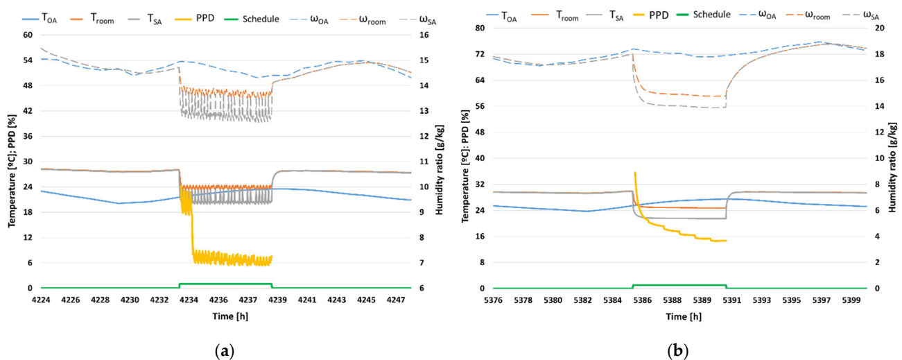
Figure 5. Temperature and humidity. DX system in Lampedusa. (a) Typical summer day and (b) Severe summer day.
