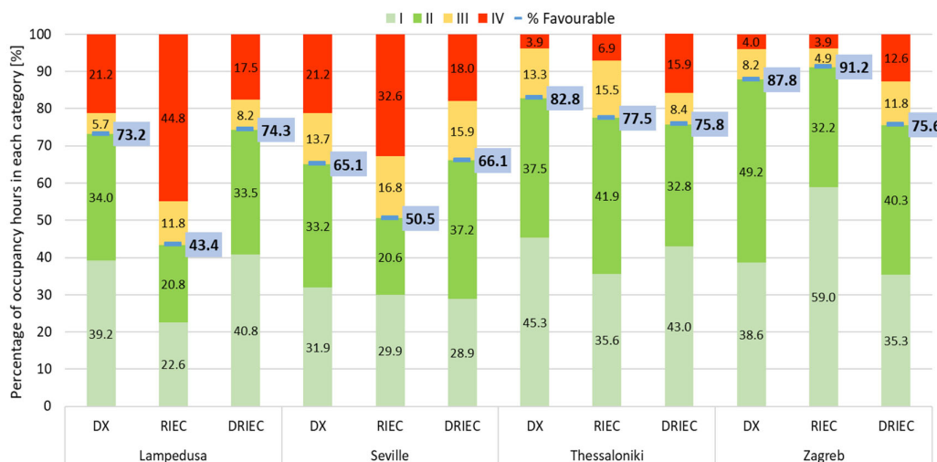
Figure 8. Annual thermal comfort results. Percentage of occupancy hours in each category.
