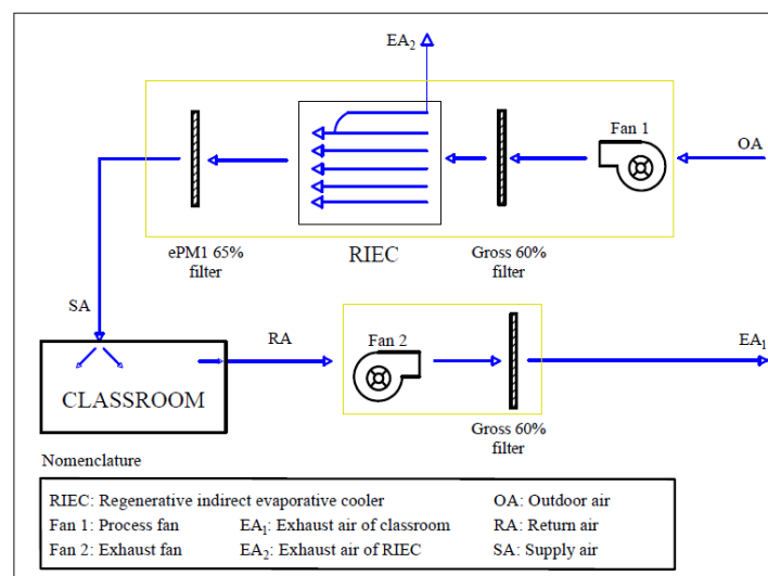
Figure 2. Schematic of the RIEC system.
