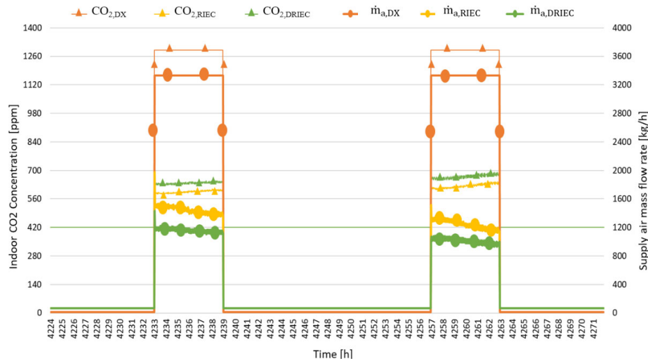
Figure 9. Indoor CO 2 concentration and supply air mass flow rate. DX, RIEC and DRIEC systems in Lampedusa in two representative summer days.
