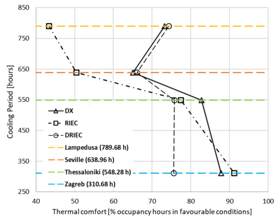
Figure 16. Influence of climatic severity on thermal comfort indicator.
