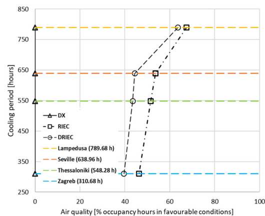
Figure 17. Influence of climatic severity on air quality indicator.
