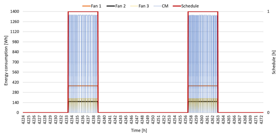
Figure 11. Energy consumption. DX system in Lampedusa in two representative summer days.
