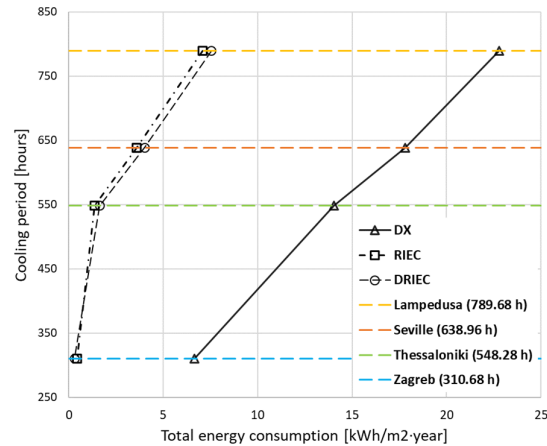
Figure 18. Influence of climatic severity on energy consumption indicator.
