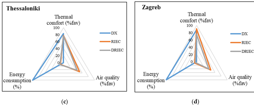
Figure 19. Radar chart. Systems and climate zones comparison (a) Lampedusa; (b) Seville; (c) Thessaloniki and (d) Zagreb.
