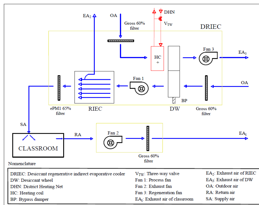
Figure 3. Schematic of the DRIEC system.
