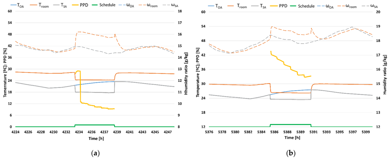
Figure 6. Temperature and humidity. RIEC system in Lampedusa. (a) Typical summer day and (b) Severe summer day.
