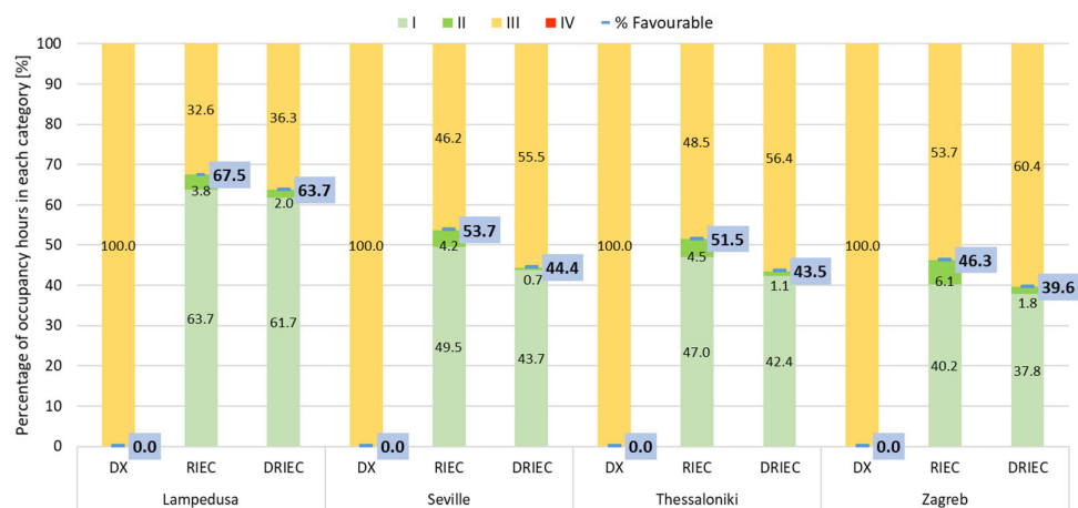
Figure 10. Annual air quality results. Percentage of occupancy hours in each category.
