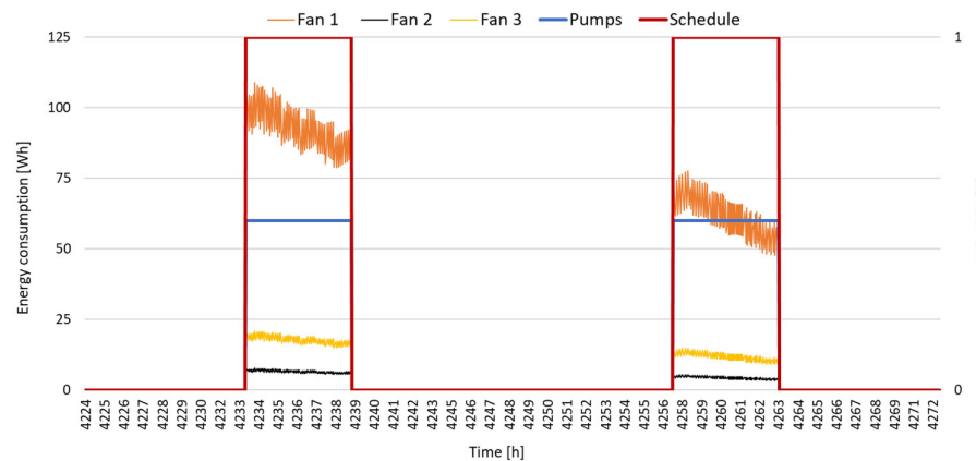
Figure 13. Energy consumption. DRIEC system in Lampedusa in two representative summer days.
