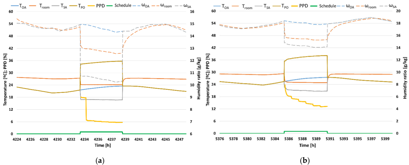
Figure 7. Temperature and humidity. DRIEC system in Lampedusa. (a) Typical summer day and (b) Severe summer day.
