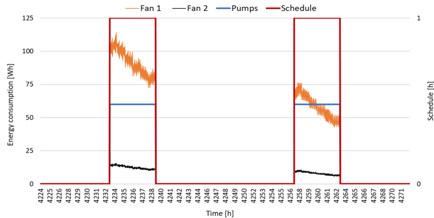
Figure 12. Energy consumption. RIEC system in Lampedusa in two representative summer days.
