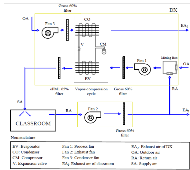
Figure 1. Schematic of the DX system.
