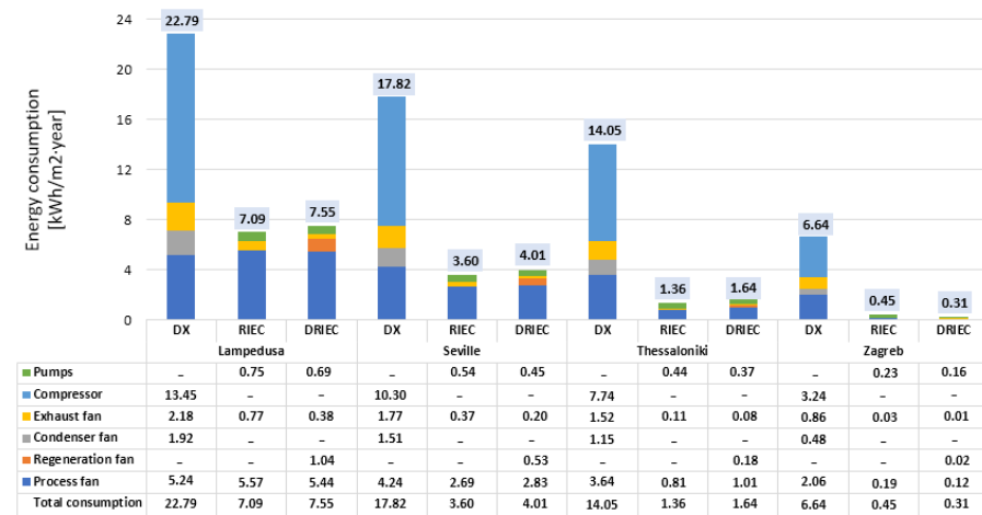
Figure 14. Annual energy consumption results.
