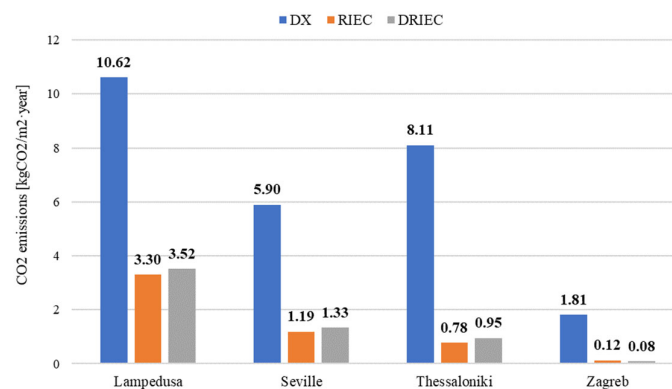
Figure 15. Annual CO 2 emissions results.
