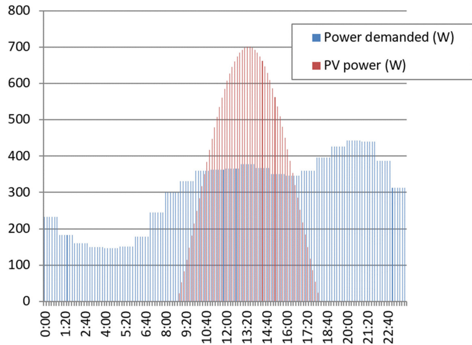
Figure 4. Production-demand curve of a PV installation with self-consumption.
