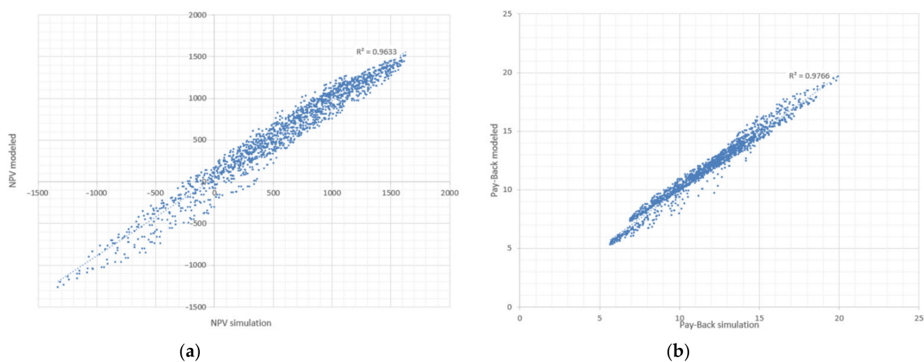
Figure 10. (a) Comparison of NPV obtained with the proposed model (Equation (32)) versus that obtained by simulation; (b) Comparison of Pay - back obtained with the proposed model (Equation (33)) versus that obtained by simulation.
