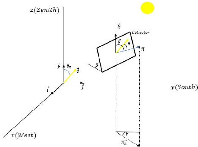
Figure 2. Vector magnitudes characteristic of the geometry of the collectors of a self-consumption PV plant.
