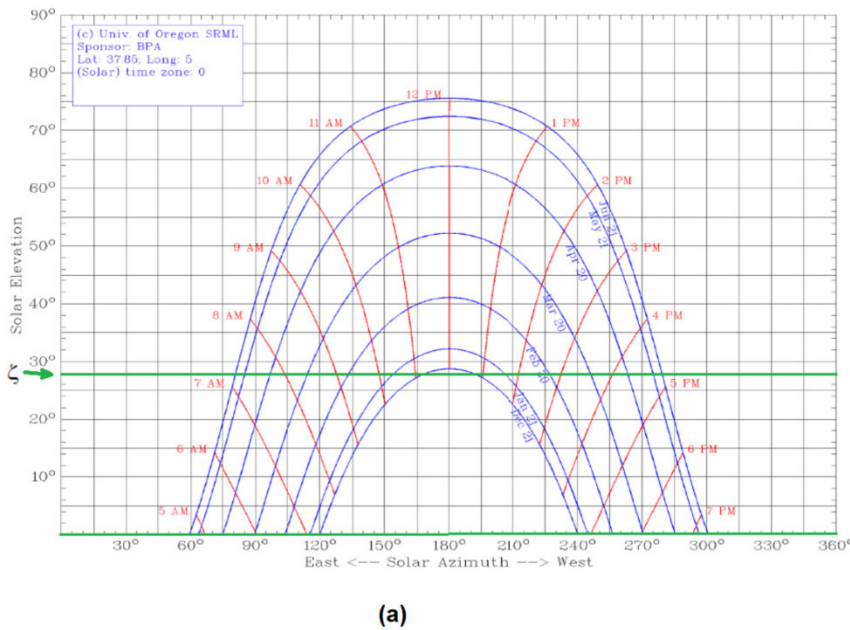
Figure 3. Obstruction profiles: (a) cylindrical chart representation; (b) geometric representation.
