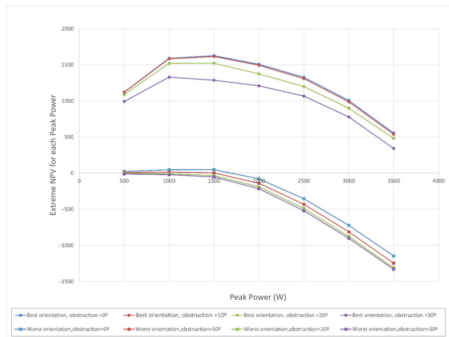
Figure 7. NPV depending on peak power and degree of obstruction for optimal orientation and worst orientation.
