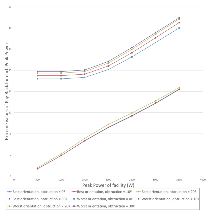
Figure 9. Achievable Pay – back depending on peak power and degree of obstruction.
