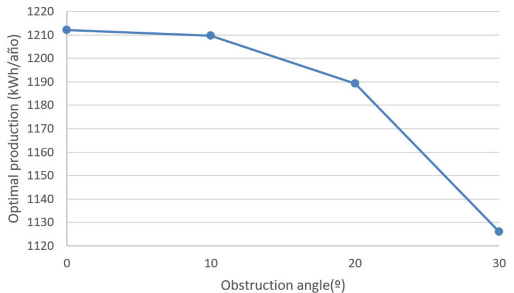
Figure 6. Optimal production reduction in a 1000 Wp plant depending on the degree of obstruction.
