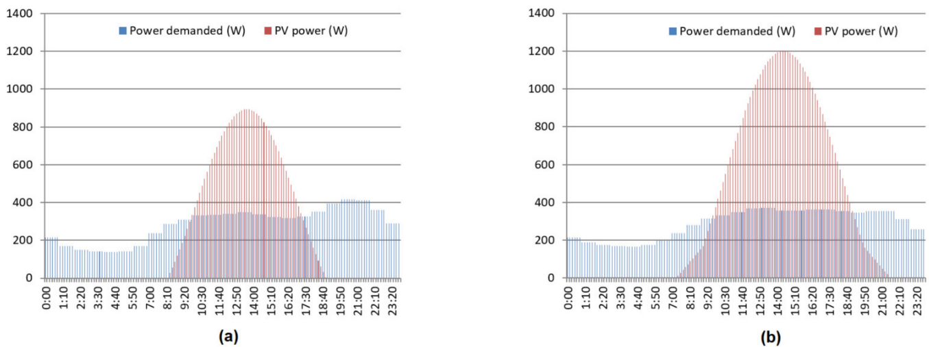
Figure 5. Hourly profiles of demand in: (a) January and (b) July [36].
