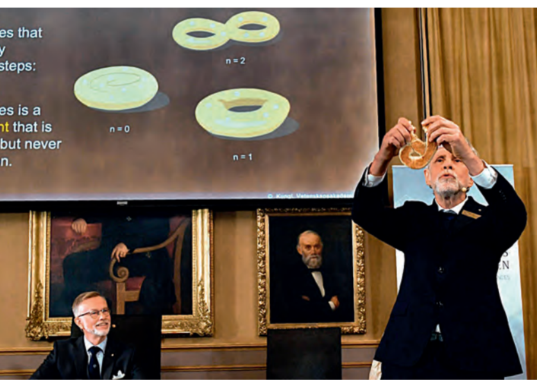
Figure 1. Torus T .
