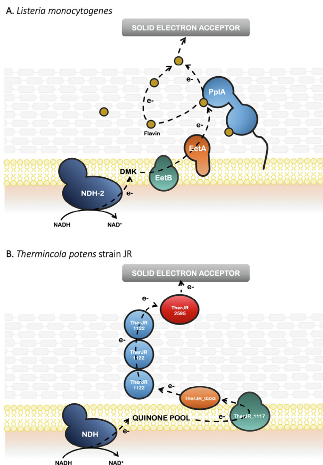
Fig. 2. Model for the proposed EET processes pathway of L. monocytogenes (A) (adapted from [16]) and T. potens (B) (adapted from [29]).
