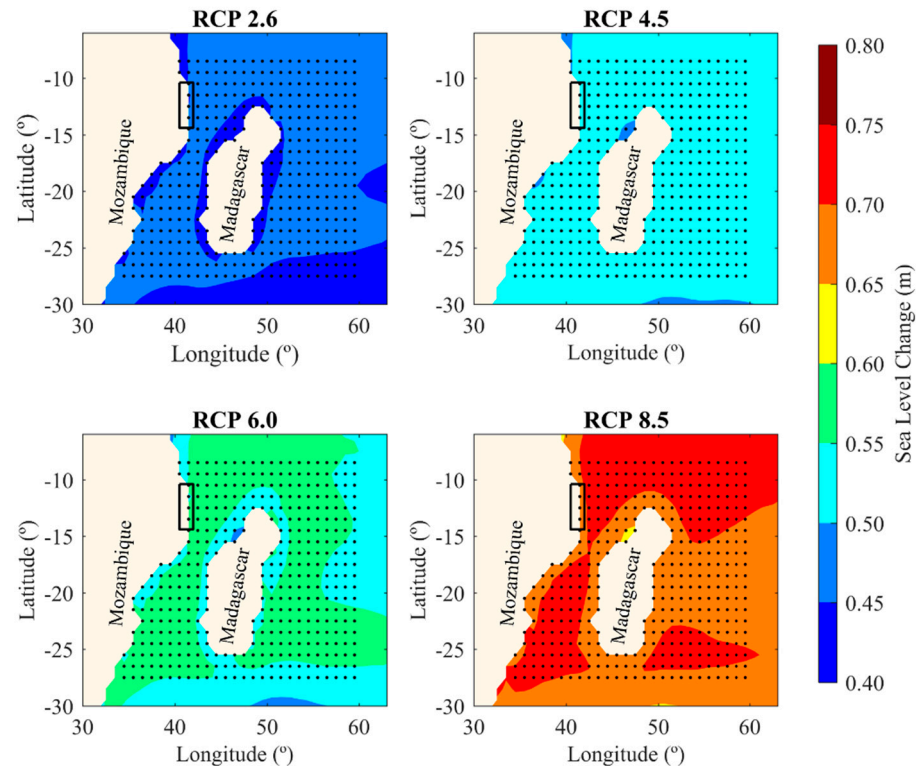
Figure 3. Sea-level change (m) around the Mozambican coast during 2081–2100 for each RCP scenario relative to 1980–2005. The black dots represent the grid points considered to compute the local mean.
