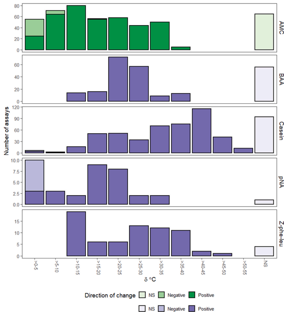
Fig. 4. Number of assays for each \delta temperature ( ^{\circ}\text{C} ) between the assay temperature and mean annual temperature (MAT) ( n of studies = 173, 99, 262, 22, 22, for AMC, BAA, casein, pNA and Z-phe-leu substrates, respectively). Colorimetric substrates are shown in purple and fluorimetric substrates are shown in green. (For interpretation of the references to color in this figure legend, the reader is referred to the Web version of this article.)
