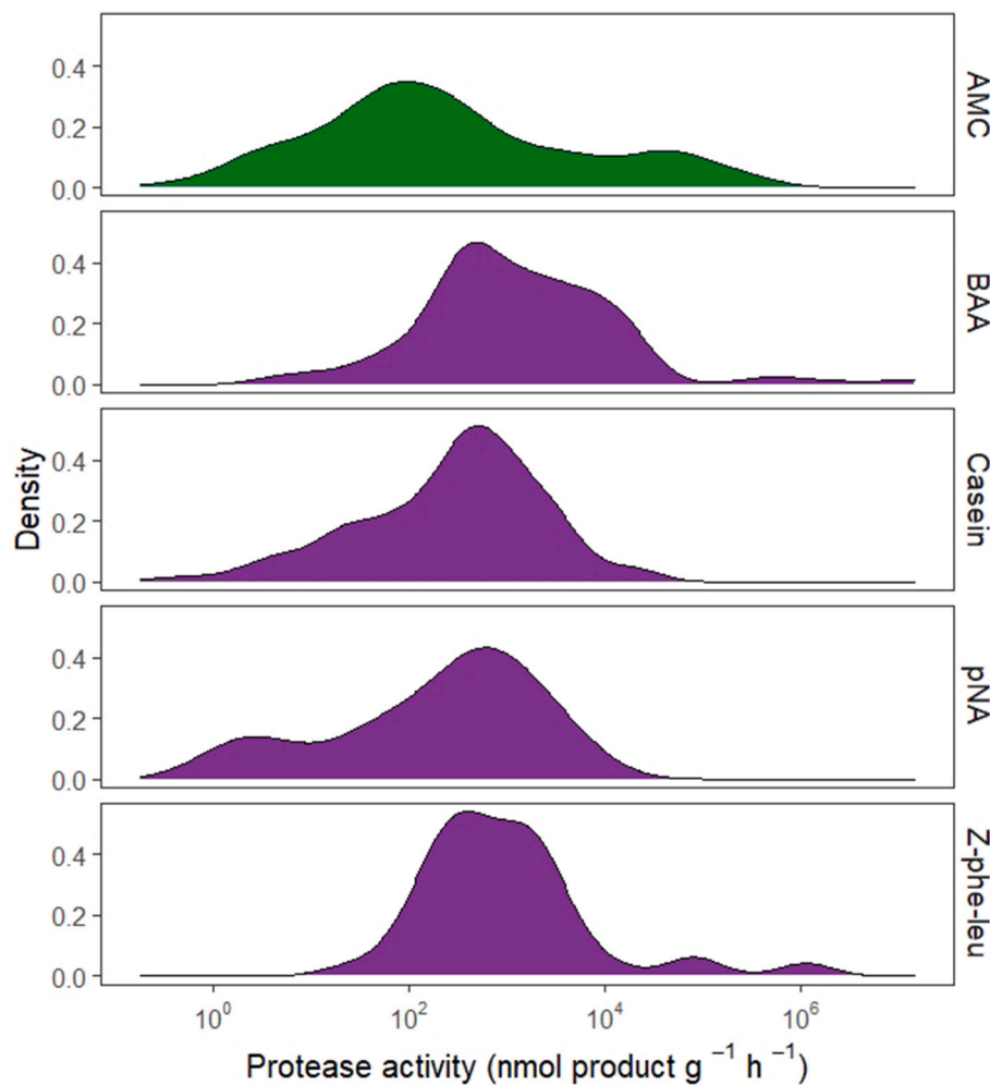
Fig. 5. Density distribution of the mean soil protease activity ( \text{nmol product g}^{-1} \text{h}^{-1} ) on a \log_{10} scale for each substrate with outliers removed ( n of studies = 162, 98, 244, 22 and 22 for AMC, BAA, casein, pNA and Z-phe-leu, respectively). Outliers were removed by estimating the maximum activity possible for the assay based on the amount of substrate added (i.e. theoretically impossible values where the reported protease activity exceeded the amount of substrate added were not deemed scientifically credible and were thus omitted). Colorimetric substrates are shown in purple and fluorimetric substrates are shown in green. (For interpretation of the references to color in this figure legend, the reader is referred to the Web version of this article.)
