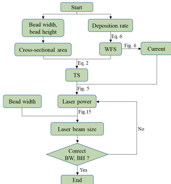
Fig. 16. Procedure for bead shape control in wire based PTA-laser hybrid AM process. Note, BW and BH stand for bead width and bead height, respectively.
