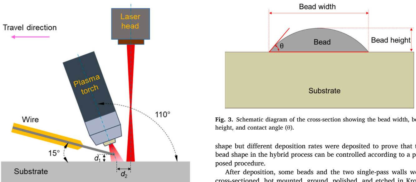
Fig. 2. Configuration used for the wire based PTA-laser hybrid AM process (side view).
