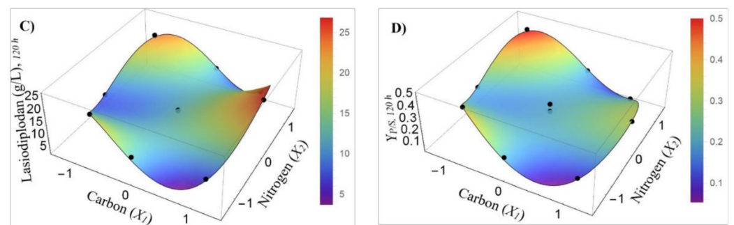
Figure 4. SCBCH and SBE interaction for lasiodiplodan production: (A) Production at 96 h; (B) Yield at 96 h; (C) Production at 120 h; (D) Yield at 120 h.
