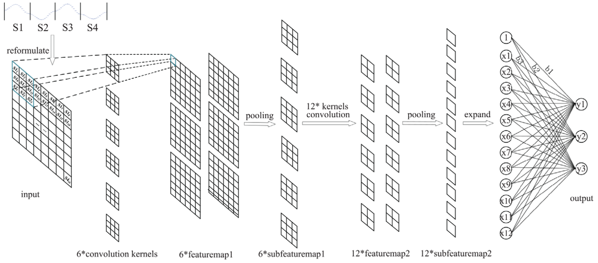
FIGURE A.1 The proposed CNN structure Note: Sixty-four sampling data corresponding to four past symbols are reformulated into 8 \times 8 matrix, then used as CNN input. Three outputs of the CNN are the predicted future symbols (1 or -1)
