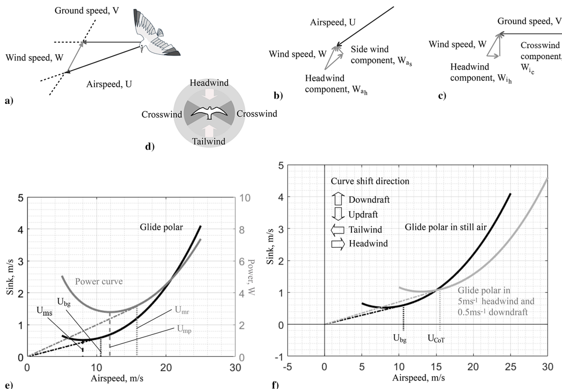
Fig. 1 Velocity diagrams and plots for calculating: a) airspeed, b) head wind in the air frame, c) headwind in the inertial frame, d) headwind [ \pm(0^\circ - 60^\circ) ], crosswind [ \pm(60^\circ - 120^\circ) ] and tailwind [ \pm(120^\circ - 180^\circ) ] angles, e) glide polar and power curve, f) COT curve shifting.
