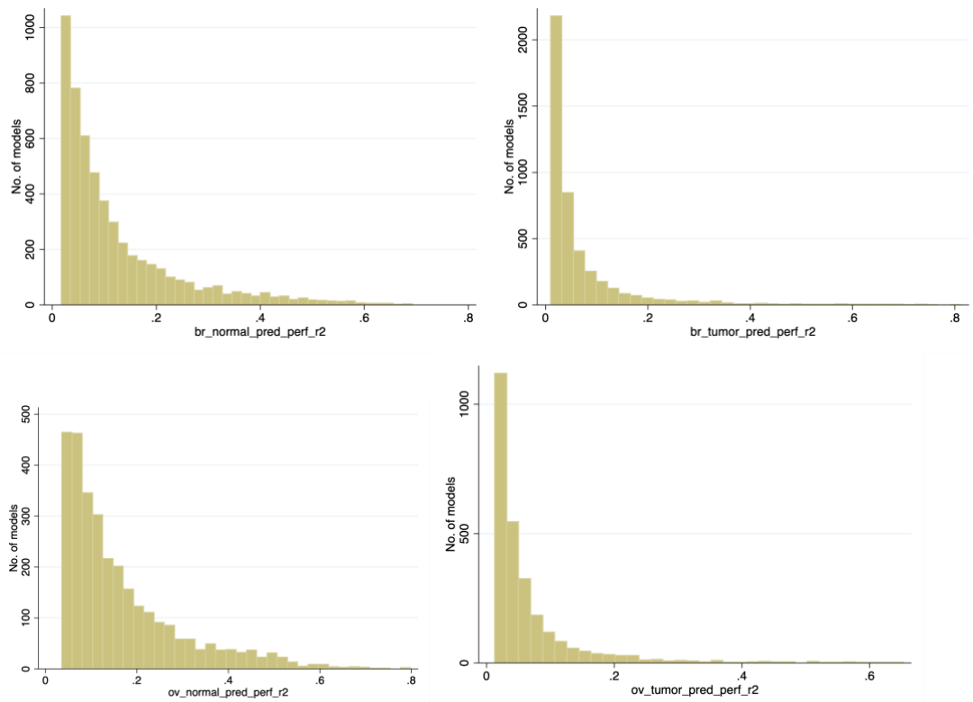
Figure S1: Prediction performance of PrediXcan models in normal and tumor breast and ovarian tissues.
