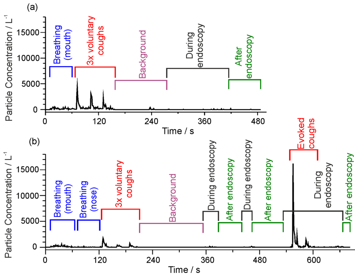
Figure 3 Continuous time series of aerosol detected during respiratory manoeuvres (tidal breathing and voluntary coughs) followed after a period of background monitoring by OGD
