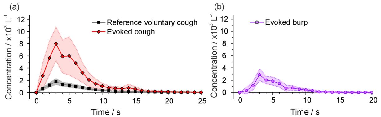
Figure 2 Mean particle concentration sampled during reference voluntary coughs (n=15 patients) overlaid with those for coughs evoked during OGD (n=9 patients) and burps observed during OGD (n=4 patients). The shaded region represents SEM.
