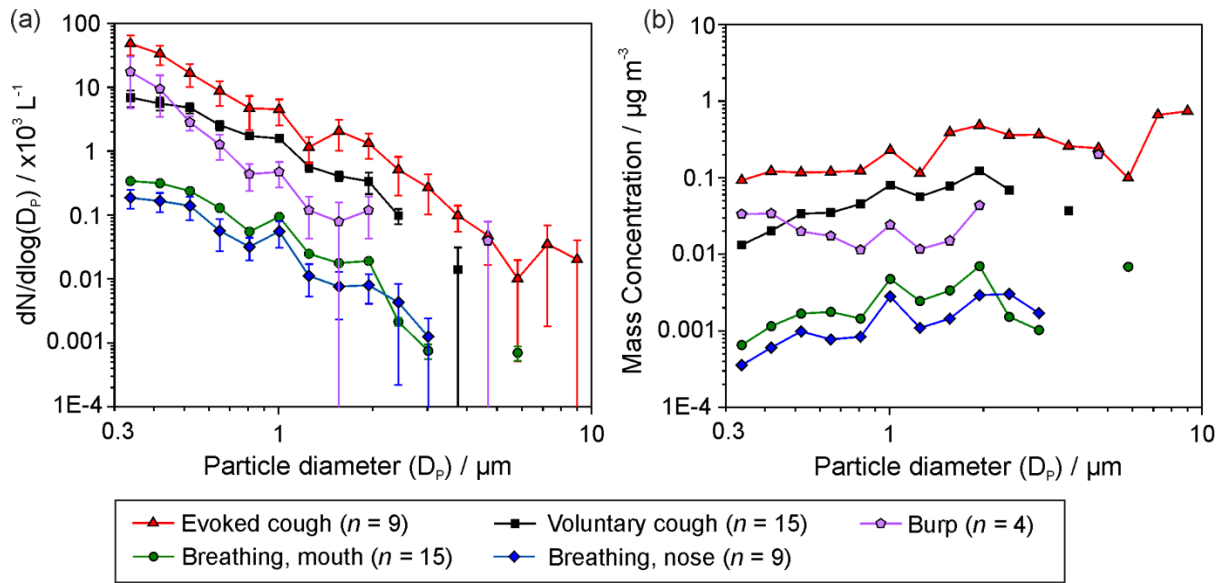
Figure 4 (a) Particle size distribution of the events. dN/d\log(D_p) is the concentration sampled within each bin normalised by the logarithm of the bin width. The error bars represent the standard error of the mean. (b) The size distribution of the average aerosol concentration generated by each activity represented in terms of a mass concentration, calculated assuming unit density.
