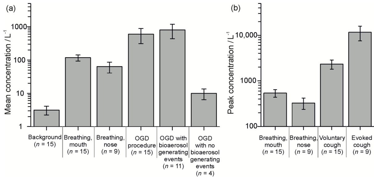
Figure 1. a) Mean particle concentrations and b) peak particle concentrations generated during the recording protocol. Note log scale for concentrations plotted as mean \pm SEM.
