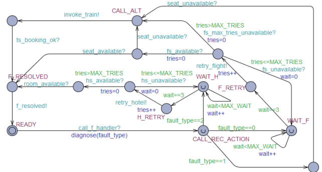
FIGURE 11. Fault handler service.
