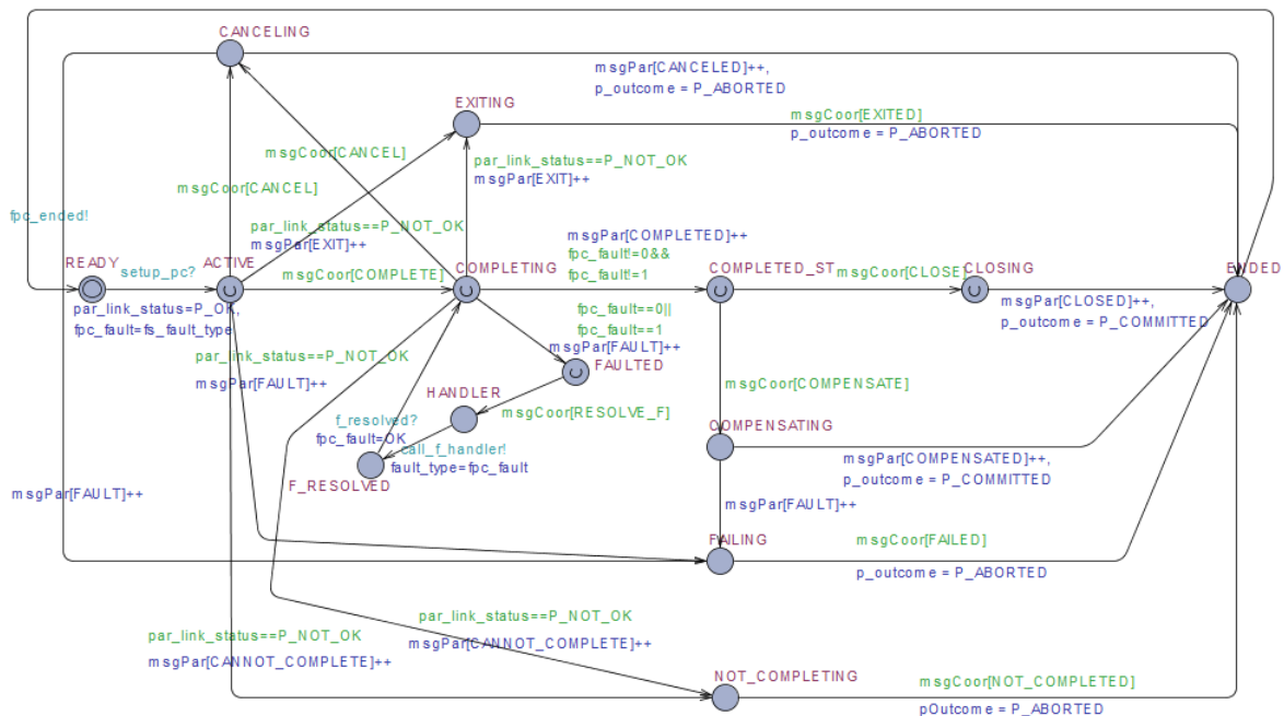
FIGURE 12. Extended WS-BA protocol.
