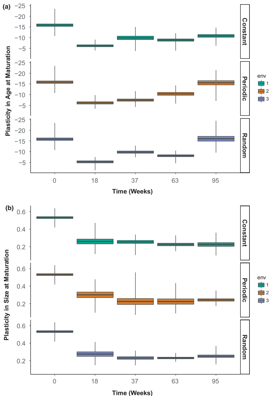
FIGURE 4 Changing prevalence of plastic genotypes over time, facets showing mean plasticity across families raised in constant, periodic, and random environments. Boxplots show the mean \pm 1 standard error, with whiskers indicating max and min. Figure (a) following initial decline shows increasing age plasticity with greatest observed in random and periodic environments which did not differ from one another. Figure (b) shows no recovery for size plasticity (linear mixed-effects model, 2 populations per treatment per timepoint)
